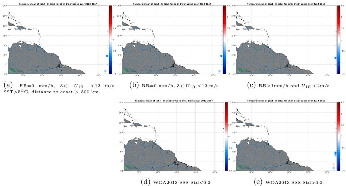
Figure 12: Temporal mean gridded over spatial boxes of size 1^{\circ}\times 1^{\circ} of \Delta\text{SSS} (SMOS L3 v2 - Daily - 0.5 Deg (CATDS-CECOS-IFREMER) - TSG-POLARSTERN) for 5 different subdatasets corresponding to:RR=0 mm/h, 3 < U_{10} < 12 m/s, SST >5^{\circ}\text{C} , distance to coast > 800 km (a), RR=0 mm/h, 3 < U_{10} < 12 m/s (b), RR >1 mm/h and U_{10} < 4 m/s (c), WOA2013 SSS Std <0.2 (d), WOA2013 SSS Std >0.2 (e).
