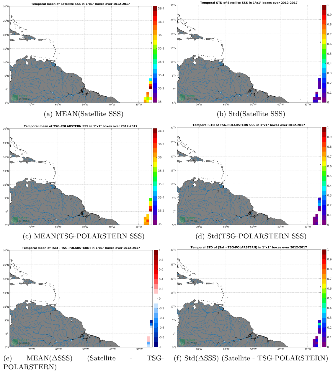
Figure 6: Temporal mean (left) and Std (right) of SSS from SMOS L3 v2 - Daily - 0.5 Deg (CATDS-CECOS-IFREMER) (top), TSG-POLARSTERN (middle), and of \Delta SSS (Satellite - TSG-POLARSTERN). Only match-up pairs are used to generate these maps.
