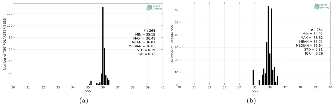
Figure 2: Histograms of SSS from TSG-POLARSTERN (a) and SMOS L3 v2 - Daily - 0.5 Deg (CATDS-CECOS-IFREMER) (b) considering all match-up pairs per bins of 0.1 over the Amazon and Orinoco river plumes Pi-MEP region and for the full satellite product period.
