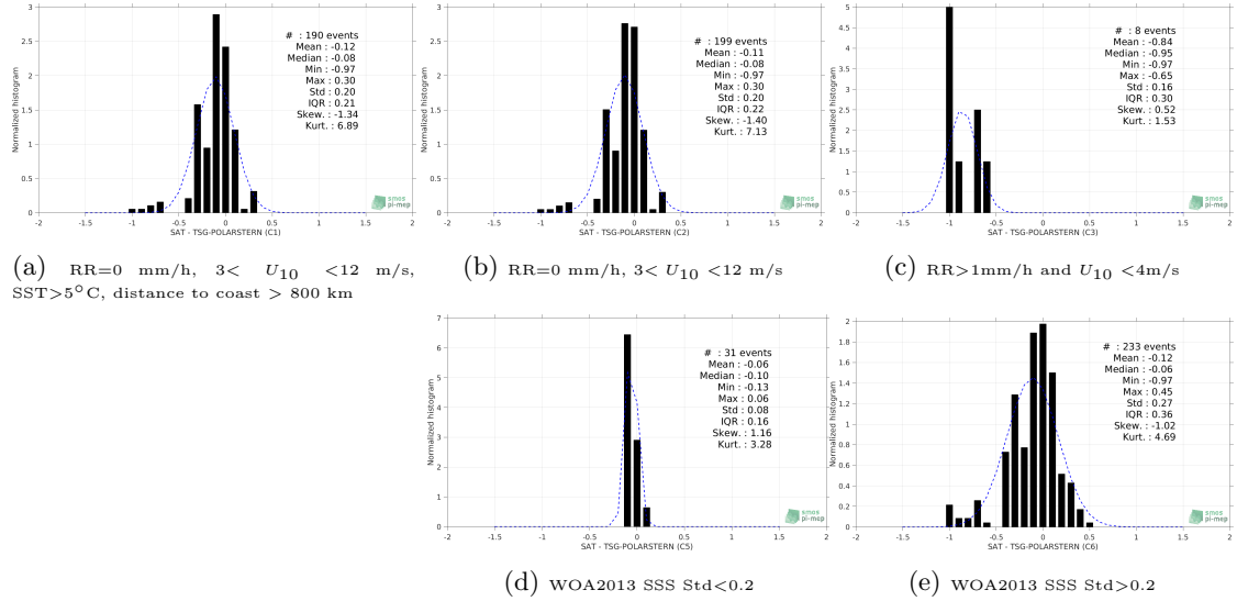
Figure 13: Normalized histogram of \Delta SSS (SMOS-L3-CATDS-CECOS-IFREMER-V2-1DAY-0.5DEG - TSG-POLARSTERN) for 5 different subdatasets corresponding to: RR=0 mm/h, 3 < U_{10} < 12 m/s, SST > 5°C, distance to coast > 800 km (a), RR=0 mm/h, 3 < U_{10} < 12 m/s (b), RR > 1mm/h and U_{10} < 4 m/s (c), WOA2013 SSS Std < 0.2 (d), WOA2013 SSS Std > 0.2 (e).
