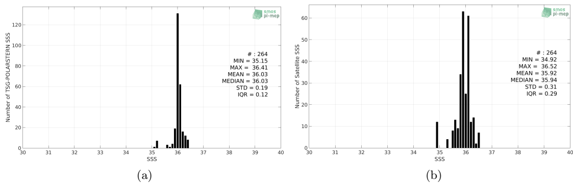
Figure 2: Histograms of SSS from TSG-POLARSTERN (a) and SMOS-L3-CATDS-CECOS-IFREMER-V2-1DAY-0.5DEG (b) considering all match-up pairs per bins of 0.1 over the Amazon and Orinoco river plumes Pi-MEP region and for the full satellite product period.
