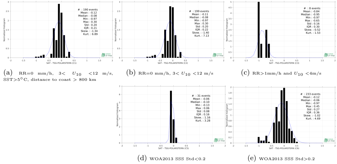
Figure 13: Normalized histogram of \Delta\text{SSS} (SMOS-L3-CATDS-CECOS-IFREMER-V2-1DAY-0.5DEG - TSG-POLARSTERN) for 5 different subdatasets corresponding to: RR=0 mm/h, 3 < U_{10} < 12 m/s, SST > 5^\circ\text{C} , distance to coast > 800 km (a), RR=0 mm/h, 3 < U_{10} < 12 m/s (b), RR > 1\text{mm/h} and U_{10} < 4\text{m/s} (c), WOA2013 SSS Std < 0.2 (d), WOA2013 SSS Std > 0.2 (e).
