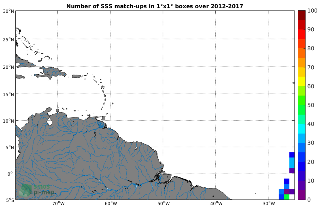
Figure 4: Number of SSS match-ups between TSG-POLARSTERN SSS and the SMOS-L3-CATDS-CECOS-IFREMER-V2-1DAY-0.5DEG SSS product for the Amazon and Orinoco river plumes Pi-MEP region over 1^\circ \times 1^\circ boxes and for the full satellite product period.
