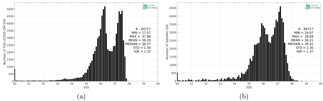
Figure 2: Histograms of SSS from TSG-LEGOS-DM (a) and SMOS L3 v2 - Daily - 0.5 Deg (CATDS-CECOS-IFREMER) (b) considering all match-up pairs per bins of 0.1 over the Amazon and Orinoco river plumes Pi-MEP region and for the full satellite product period.
