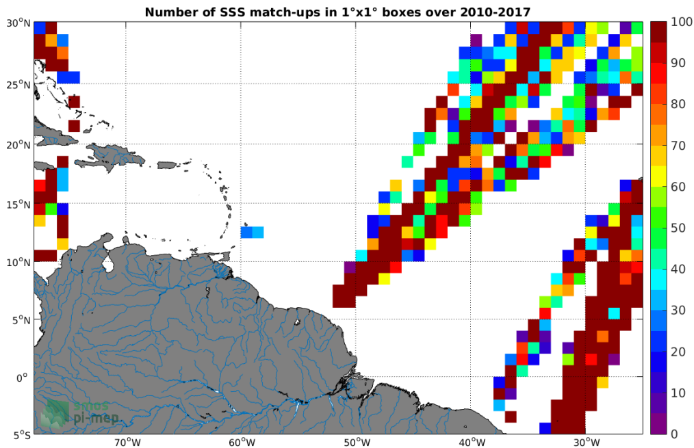
Figure 4: Number of SSS match-ups between TSG-LEGOS-DM SSS and the SMOS L3 v2 - Daily - 0.5 Deg (CATDS-CECOS-IFREMER) SSS product for the Amazon and Orinoco river plumes Pi-MEP region over 1°x1° boxes and for the full satellite product period.
