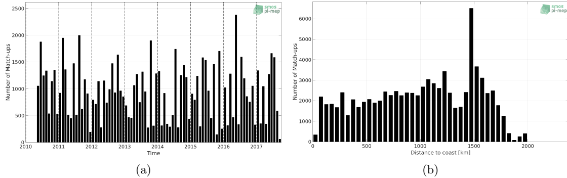
Figure 1: Number of match-ups between TSG-LEGOS-DM and SMOS L3 v2 - Daily - 0.5 Deg (CATDS-CECOS-IFREMER) SSS as a function of time (a) and as function of the distance to coast (b) over the Amazon and Orinoco river plumes Pi-MEP region and for the full satellite product period.
