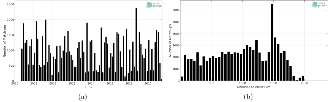
Figure 1: Number of match-ups between TSG-LEGOS-DM and SMOS-L3-CATDS-CECOS-IFREMER-V2-1DAY-0.5DEG SSS as a function of time (a) and as function of the distance to coast (b) over the Amazon and Orinoco river plumes Pi-MEP region and for the full satellite product period.
