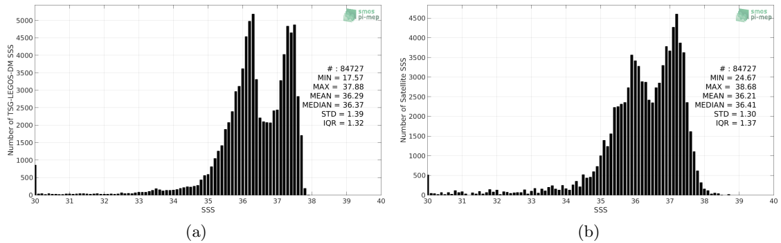
Figure 2: Histograms of SSS from TSG-LEGOS-DM (a) and SMOS-L3-CATDS-CECOS-IFREMER-V2-1DAY-0.5DEG (b) considering all match-up pairs per bins of 0.1 over the Amazon and Orinoco river plumes Pi-MEP region and for the full satellite product period.
