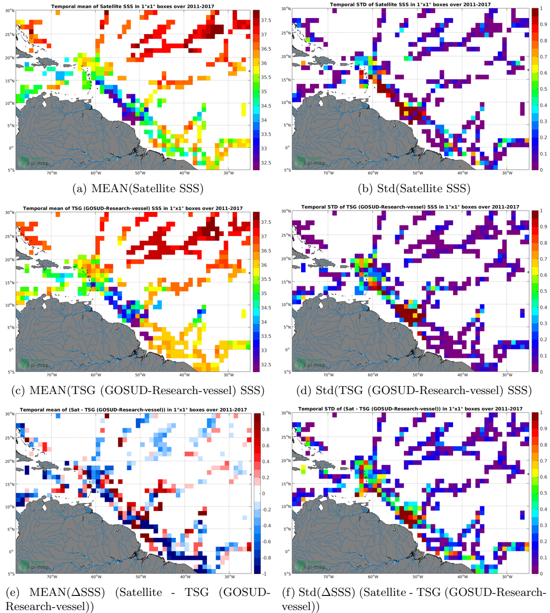
Figure 6: Temporal mean (left) and Std (right) of SSS from SMOS SSS L3 v2 - Daily - 0.5 Deg (CATDS-CECOS-IFREMER) (top), TSG (GOSUD-Research-vessel) (middle), and of \Delta SSS (Satellite - TSG (GOSUD-Research-vessel)). Only match-up pairs are used to generate these maps.
