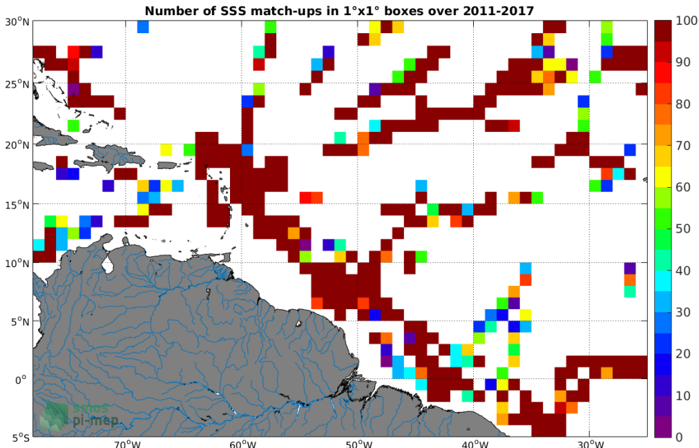
Figure 4: Number of SSS match-ups between TSG (GOSUD-Research-vessel) SSS and the SMOS SSS L3 v2 - Daily - 0.5 Deg (CATDS-CECOS-IFREMER) SSS product for the Amazon and Orinoco river plumes Pi-MEP region over 1^\circ \times 1^\circ boxes and for the full satellite product period.
