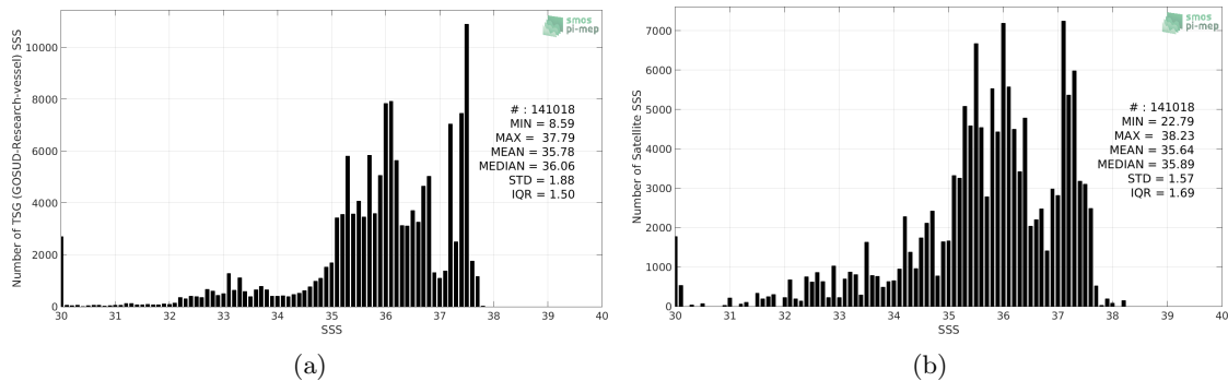
Figure 2: Histograms of SSS from TSG (GOSUD-Research-vessel) (a) and SMOS SSS L3 v2 - Daily - 0.5 Deg (CATDS-CECOS-IFREMER) (b) considering all match-up pairs per bins of 0.1 over the Amazon and Orinoco river plumes Pi-MEP region and for the full satellite product period.
