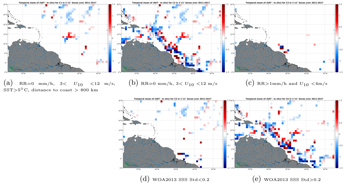
Figure 12: Temporal mean gridded over spatial boxes of size 1^\circ \times 1^\circ of \Delta SSS (SMOS SSS L3 v2 - Daily - 0.5 Deg (CATDS-CECOS-IFREMER) - TSG (GOSUD-Research-vessel)) for 5 different subdatasets corresponding to:RR=0 mm/h, 3 < U_{10} < 12 m/s, SST >5^\circ\text{C} , distance to coast > 800 km (a), RR=0 mm/h, 3 < U_{10} < 12 m/s (b), RR >1 mm/h and U_{10} < 4 m/s (c), WOA2013 SSS Std <0.2 (d), WOA2013 SSS Std >0.2 (e).
