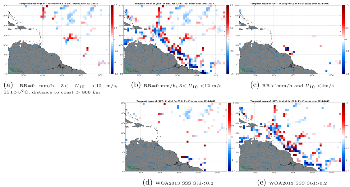
Figure 12: Temporal mean gridded over spatial boxes of size 1^{\circ}\times 1^{\circ} of \Delta SSS (SMOS L3 v2 - Daily - 0.5 Deg (CATDS-CECOS-IFREMER) - TSG-GOSUD-Research-vessel) for 5 different subdatasets corresponding to:RR=0 mm/h, 3 < U_{10} < 12 m/s, SST >5^{\circ}\text{C} , distance to coast > 800 km (a), RR=0 mm/h, 3 < U_{10} < 12 m/s (b), RR >1 mm/h and U_{10} < 4 m/s (c), WOA2013 SSS Std <0.2 (d), WOA2013 SSS Std >0.2 (e).
