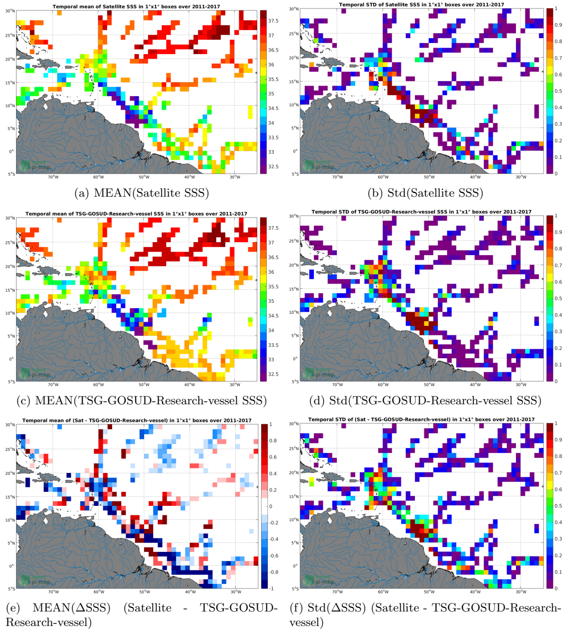
Figure 6: Temporal mean (left) and Std (right) of SSS from SMOS L3 v2 - Daily - 0.5 Deg (CATDS-CECOS-IFREMER) (top), TSG-GOSUD-Research-vessel (middle), and of \Delta SSS (Satellite - TSG-GOSUD-Research-vessel). Only match-up pairs are used to generate these maps.
