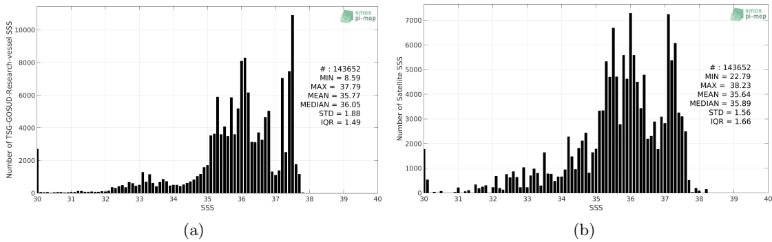
Figure 2: Histograms of SSS from TSG-GOSUD-Research-vessel (a) and SMOS L3 v2 - Daily - 0.5 Deg (CATDS-CECOS-IFREMER) (b) considering all match-up pairs per bins of 0.1 over the Amazon and Orinoco river plumes Pi-MEP region and for the full satellite product period.
