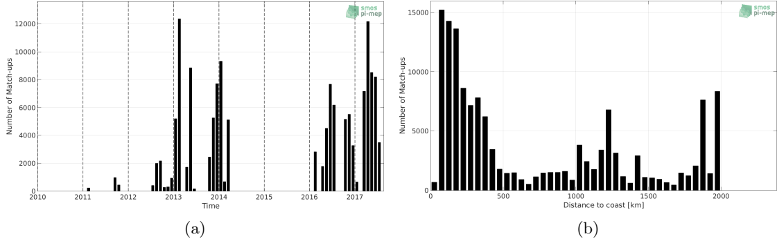
Figure 1: Number of match-ups between TSG-GOSUD-Research-vessel and SMOS L3 v2 - Daily - 0.5 Deg (CATDS-CECOS-IFREMER) SSS as a function of time (a) and as function of the distance to coast (b) over the Amazon and Orinoco river plumes Pi-MEP region and for the full satellite product period.
