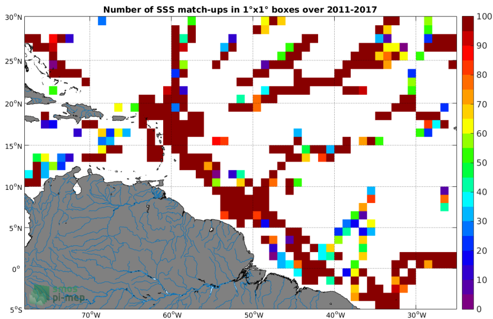
Figure 4: Number of SSS match-ups between TSG-GOSUD-Research-vessel SSS and the SMOS L3 v2 - Daily - 0.5 Deg (CATDS-CECOS-IFREMER) SSS product for the Amazon and Orinoco river plumes Pi-MEP region over 1^\circ \times 1^\circ boxes and for the full satellite product period.
