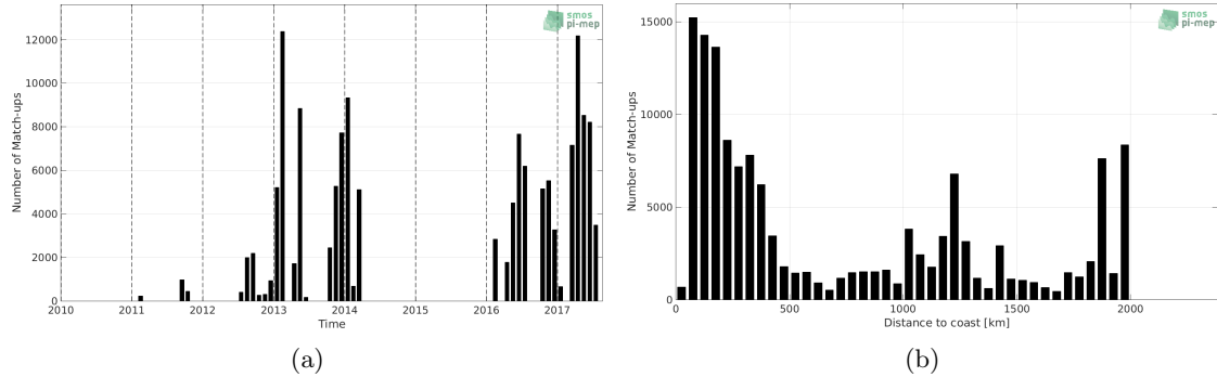
Figure 1: Number of match-ups between TSG-GOSUD-Research-vessel and SMOS-L3-CATDS-CECOS-IFREMER-V2-1DAY-0.5DEG SSS as a function of time (a) and as function of the distance to coast (b) over the Amazon and Orinoco river plumes Pi-MEP region and for the full satellite product period.
