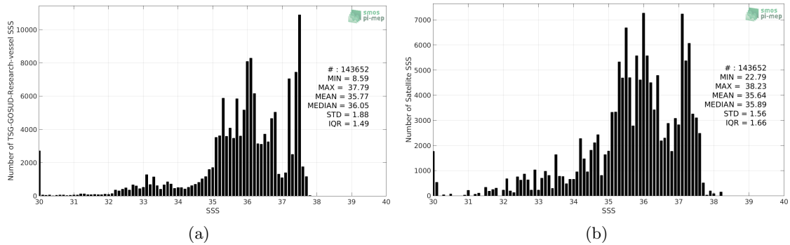
Figure 2: Histograms of SSS from TSG-GOSUD-Research-vessel (a) and SMOS-L3-CATDS-CECOS-IFREMER-V2-1DAY-0.5DEG (b) considering all match-up pairs per bins of 0.1 over the Amazon and Orinoco river plumes Pi-MEP region and for the full satellite product period.
