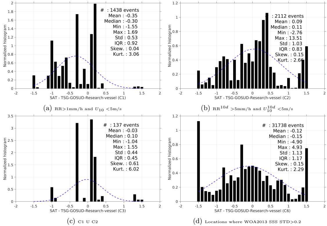
Figure 13: Normalized histogram of \Delta\text{SSS} (SMOS-L3-CATDS-CECOS-IFREMER-V2-1DAY-0.5deg - TSG-GOSUD-Research-vessel) for 6 different subdatasets corresponding to: \text{RR} > 1\text{mm/h} and U_{10} < 5\text{m/s} (a), \text{RR}^{10d} > 5\text{mm/h} and U_{10}^{10d} < 5\text{m/s} (b), C1 U C2 (c), Locations where WOA2013 SSS STD > 0.2 (d).
