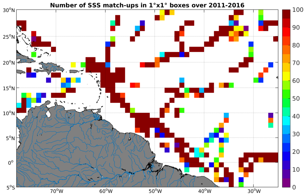
Figure 4: Number of SSS match-ups between TSG-GOSUD-Research-vessel SSS and the SMOS-L3-CATDS-CECOS-IFREMER-V2-1DAY-0.5deg SSS product for the Amazon and Orinoco river plumes Pi-MEP region over 1^\circ \times 1^\circ boxes and for the full satellite product period.
