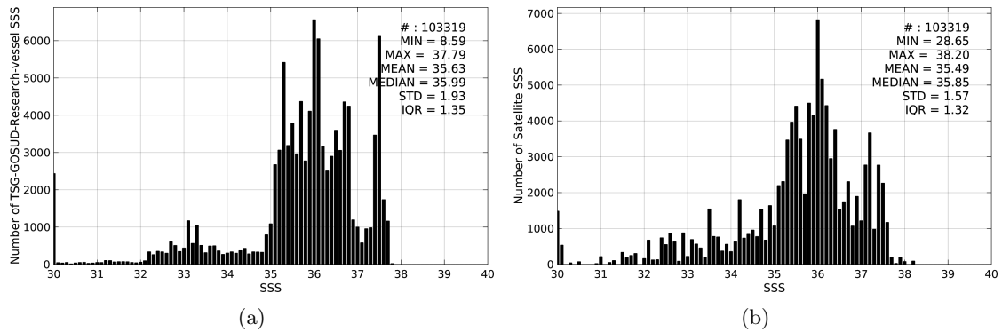
Figure 2: Histograms of SSS from TSG-GOSUD-Research-vessel (a) and SMOS-L3-CATDS-CECOS-IFREMER-V2-1DAY-0.5deg (b) considering all match-up pairs per bins of 0.1 over the Amazon and Orinoco river plumes Pi-MEP region and for the full satellite product period.
