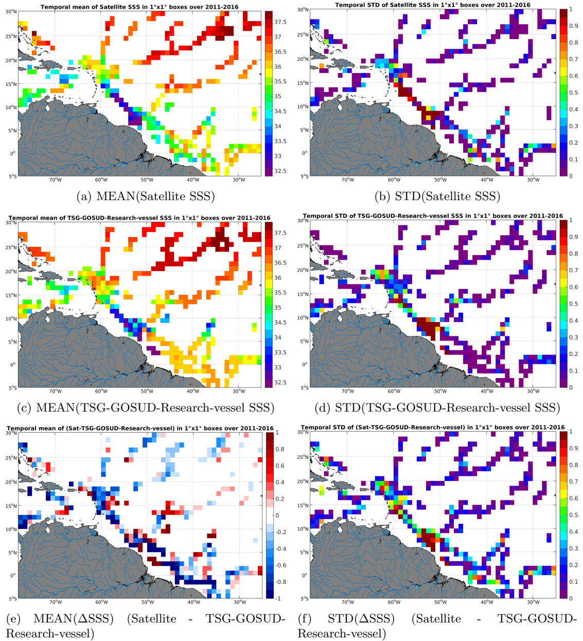
Figure 6: Temporal mean (left) and STD (right) of SSS from SMOS-L3-CATDS-CECOS-IFREMER-V2-1DAY-0.5deg (top), TSG-GOSUD-Research-vessel (middle), and of \Delta SSS (Satellite - TSG-GOSUD-Research-vessel). Only match-up pairs are used to generate these maps.
