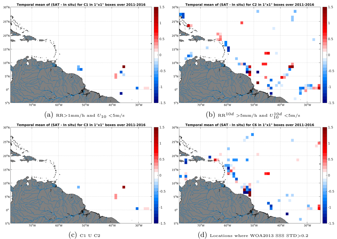
Figure 12: Temporal mean gridded over spatial boxes of size 1^\circ \times 1^\circ of \Delta SSS (SMOS-L3-CATDS-CECOS-IFREMER-V2-1DAY-0.5deg - TSG-GOSUD-Research-vessel) for 4 different subdatasets corresponding to:RR >1 mm/h and U_{10} < 5 m/s (a), RR 10d > 5 mm/h and U_{10}^{10d} < 5 m/s (b), C1 U C2 (c),Locations where WOA2013 SSS STD >0.2 (d).
