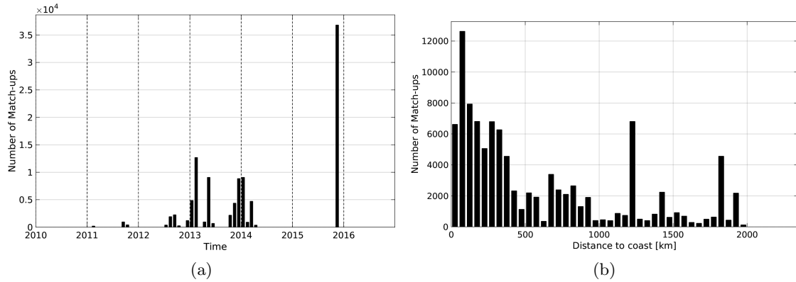
Figure 1: Number of match-ups between TSG-GOSUD-Research-vessel and SMOS-L3-CATDS-CECOS-IFREMER-V2-1DAY-0.5deg SSS as a function of time (a) and as function of the distance to coast (b) over the Amazon and Orinoco river plumes Pi-MEP region and for the full satellite product period.
