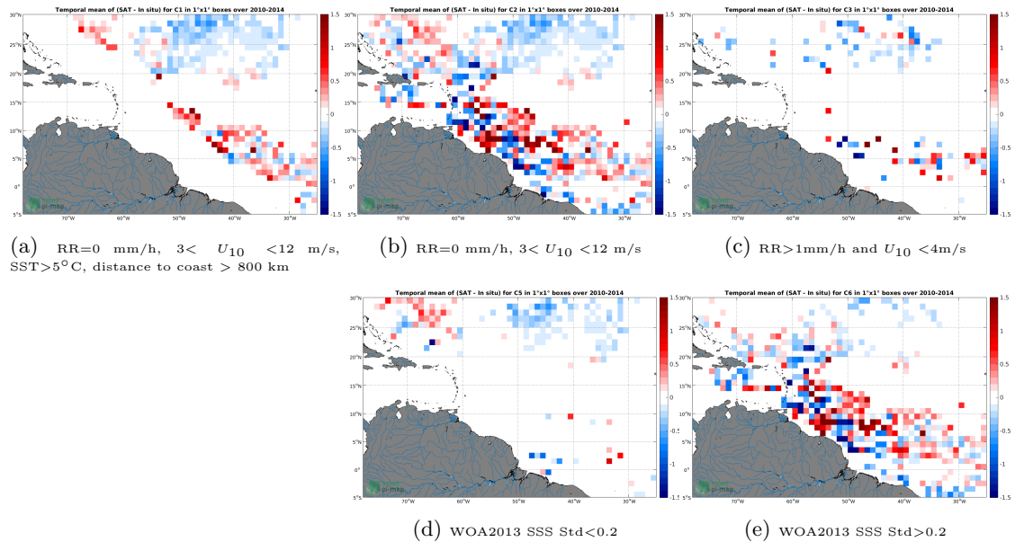
Figure 11: Temporal mean gridded over spatial boxes of size 1^{\circ}\times 1^{\circ} of \Delta\text{SSS} (SMOS SSS L3 v2 - Daily - 0.5 Deg (CATDS-CECOS-IFREMER) - Surface drifters) for 5 different subdatasets corresponding to:RR=0 mm/h, 3 < U_{10} < 12 m/s, SST >5^{\circ}\text{C} , distance to coast > 800 km (a), RR=0 mm/h, 3 < U_{10} < 12 m/s (b), RR >1 mm/h and U_{10} < 4 m/s (c), WOA2013 SSS Std <0.2 (d), WOA2013 SSS Std >0.2 (e).
