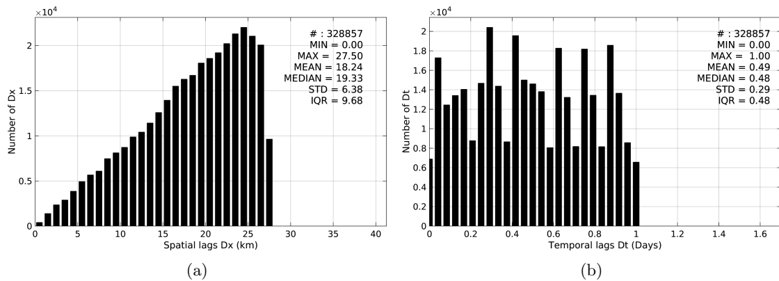
Figure 4: Histograms of the spatial (a) and temporal (b) lags between the time of the Surface drifters measurements and the date of the corresponding SMOS-L3-CATDS-CECOS-IFREMER-V2-1DAY-0.5deg SSS product.
