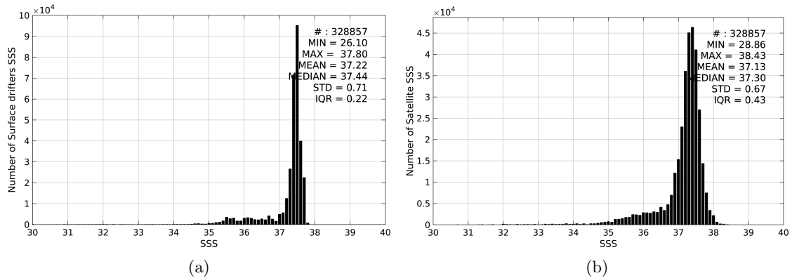
Figure 2: Histograms of SSS from Surface drifters (a) and SMOS-L3-CATDS-CECOS-IFREMER-V2-1DAY-0.5deg (b) considering all match-up pairs per bins of 0.1 over the Amazon and Orinoco river plumes Pi-MEP region and for the full satellite product period.
