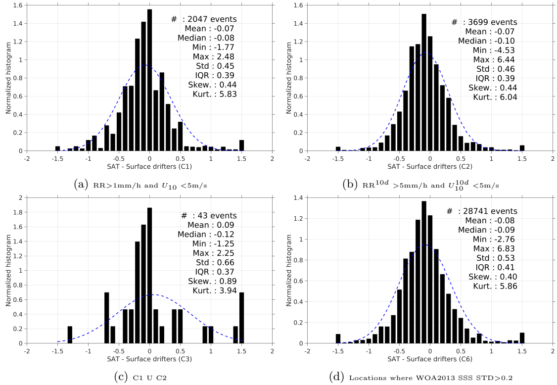
Figure 12: Normalized histogram of \Delta\text{SSS} (SMOS-L3-CATDS-CECOS-IFREMER-V2-1DAY-0.5deg - Surface drifters) for 6 different subdatasets corresponding to: \text{RR} > 1\text{mm/h} and U_{10} < 5\text{m/s} (a), \text{RR}^{10d} > 5\text{mm/h} and U_{10}^{10d} < 5\text{m/s} (b), C1 U C2 (c), Locations where WOA2013 SSS STD > 0.2 (d).
