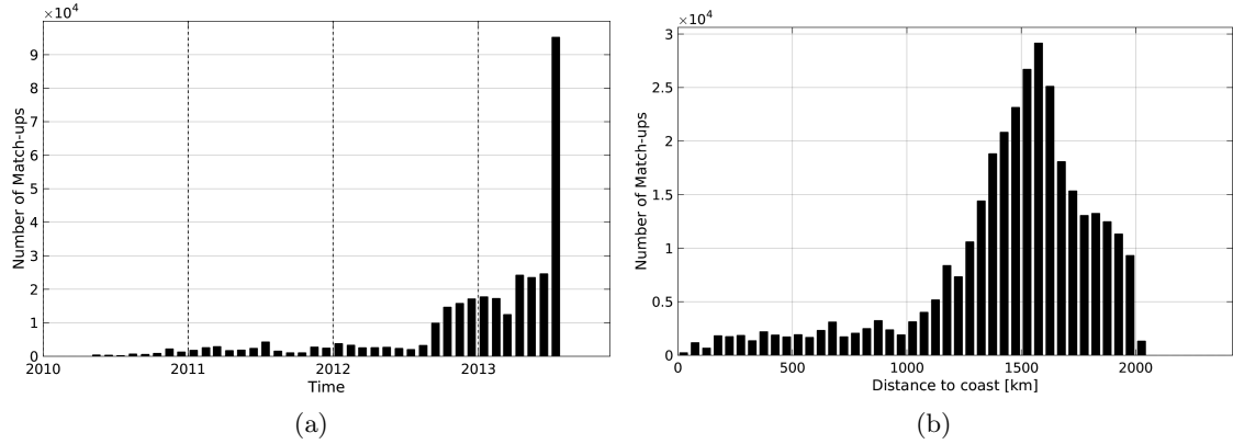
Figure 1: Number of match-ups between Surface drifters and SMOS-L3-CATDS-CECOS-IFREMER-V2-1DAY-0.5deg SSS as a function of time (a) and as function of the distance to coast (b) over the Amazon and Orinoco river plumes Pi-MEP region and for the full satellite product period.
