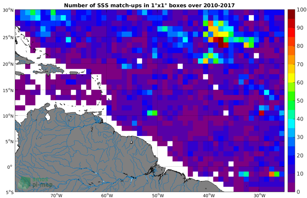
Figure 4: Number of SSS match-ups between Argo SSS and the SMOS L3 v2 - Daily - 0.5 Deg (CATDS-CECOS-IFREMER) SSS product for the Amazon and Orinoco river plumes Pi-MEP region over 1^\circ \times 1^\circ boxes and for the full satellite product period.
