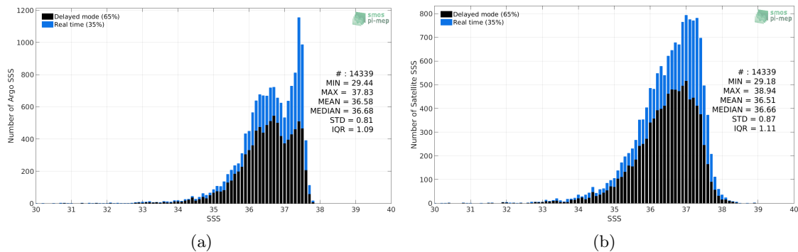
Figure 2: Histograms of SSS from Argo (a) and SMOS L3 v2 - Daily - 0.5 Deg (CATDS-CECOS-IFREMER) (b) considering all match-up pairs per bins of 0.1 over the Amazon and Orinoco river plumes Pi-MEP region and for the full satellite product period.
