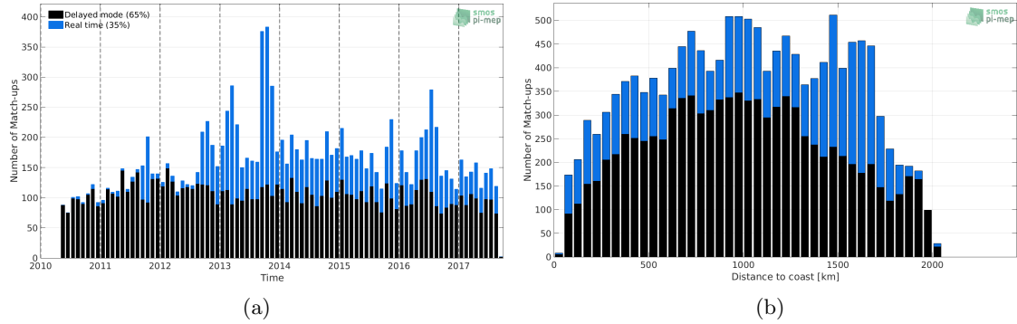
Figure 1: Number of match-ups between Argo and SMOS L3 v2 - Daily - 0.5 Deg (CATDS-CECOS-IFREMER) SSS as a function of time (a) and as function of the distance to coast (b) over the Amazon and Orinoco river plumes Pi-MEP region and for the full satellite product period.
