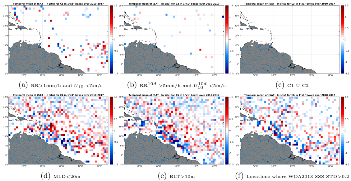
Figure 12: Temporal mean gridded over spatial boxes of size 1^\circ \times 1^\circ of \Delta SSS (SMOS-L3-CATDS-CECOS-IFREMER-V2-1DAY-0.5deg - Argo) for 6 different subdatasets corresponding to:RR>1mm/h and U_{10} < 5\text{m/s} (a), RR^{10d} > 5\text{mm/h} and U_{10}^{10d} < 5\text{m/s} (b), C1 U C2 (c),MLD<20m (d),BLT>10m (e),Locations where WOA2013 SSS STD>0.2 (f).
