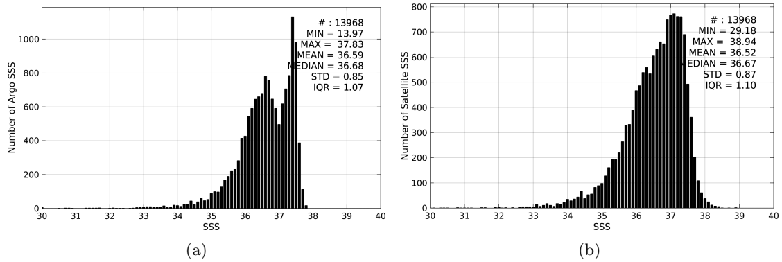
Figure 2: Histograms of SSS from Argo (a) and SMOS-L3-CATDS-CECOS-IFREMER-V2-1DAY-0.5deg (b) considering all match-up pairs per bins of 0.1 over the Amazon and Orinoco river plumes Pi-MEP region and for the full satellite product period.
