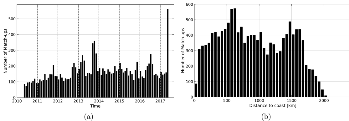
Figure 1: Number of match-ups between Argo and SMOS-L3-CATDS-CECOS-IFREMER-V2-1DAY-0.5deg SSS as a function of time (a) and as function of the distance to coast (b) over the Amazon and Orinoco river plumes Pi-MEP region and for the full satellite product period.
