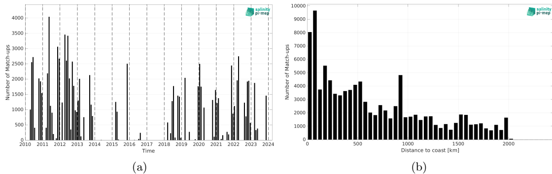
Figure 2: Number of match-ups between TSG (SAMOS) and SMOS SSS L3 v335 - Monthly - 25 km (CATDS-CPDC) SSS as a function of time (a) and as function of the distance to coast (b) over the Amazon and Orinoco river plumes Pi-MEP region and for the full satellite product period.
