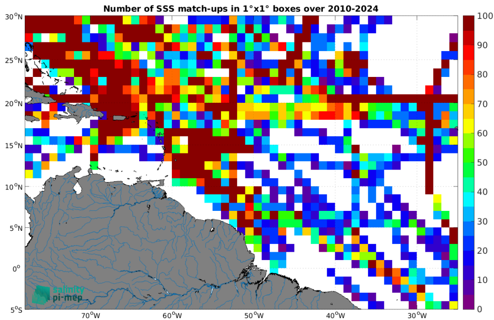
Figure 5: Number of SSS match-ups between TSG (SAMOS) SSS and the SMOS SSS L3 v335 - Monthly - 25 km (CATDS-CPDC) SSS product for the Amazon and Orinoco river plumes Pi-MEP region over 1^{\circ} \times 1^{\circ} boxes and for the full satellite product period.
