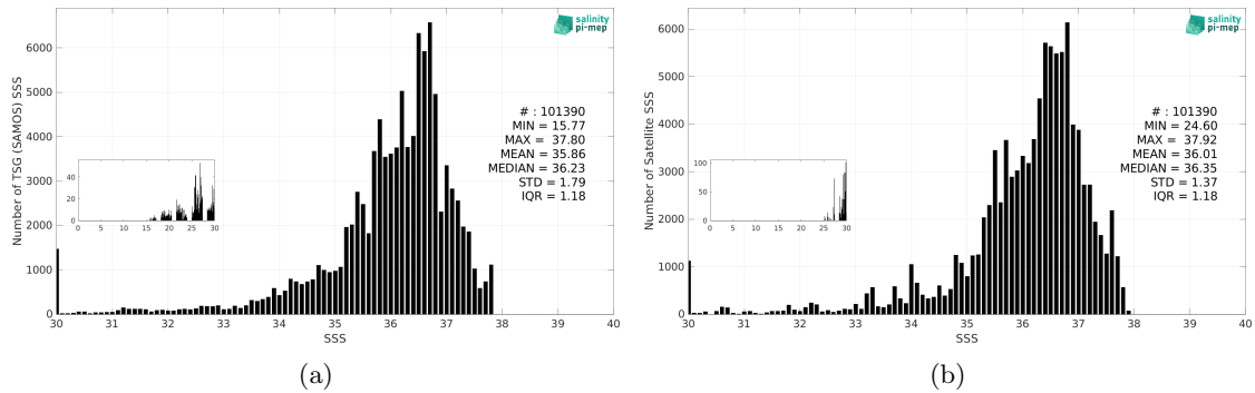
Figure 3: Histograms of SSS from TSG (SAMOS) (a) and SMOS SSS L3 v335 - Monthly - 25 km (CATDS-CPDC) (b) considering all match-up pairs per bins of 0.1 over the Amazon and Orinoco river plumes Pi-MEP region and for the full satellite product period.
