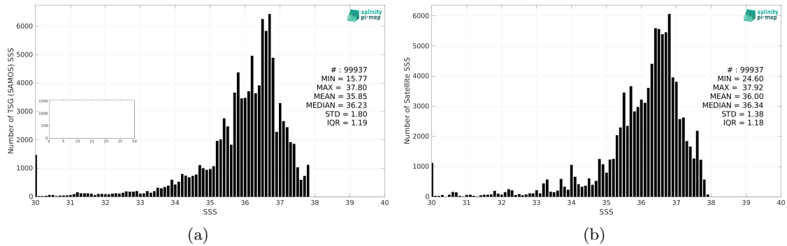
Figure 2: Histograms of SSS from TSG (SAMOS) (a) and SMOS SSS L3 v335 - Monthly - 25 km (CATDS-CPDC) (b) considering all match-up pairs per bins of 0.1 over the Amazon and Orinoco river plumes Pi-MEP region and for the full satellite product period.
