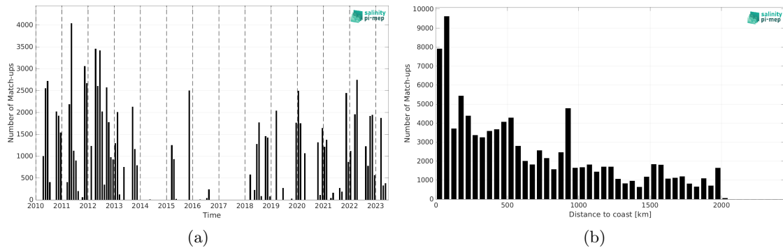
Figure 1: Number of match-ups between TSG (SAMOS) and SMOS SSS L3 v335 - Monthly - 25 km (CATDS-CPDC) SSS as a function of time (a) and as function of the distance to coast (b) over the Amazon and Orinoco river plumes Pi-MEP region and for the full satellite product period.
