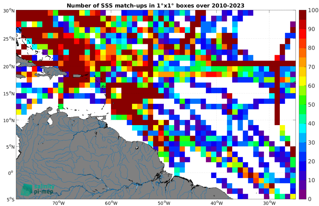
Figure 4: Number of SSS match-ups between TSG (SAMOS) SSS and the SMOS SSS L3 v335 - Monthly - 25 km (CATDS-CPDC) SSS product for the Amazon and Orinoco river plumes Pi-MEP region over 1^{\circ} \times 1^{\circ} boxes and for the full satellite product period.
