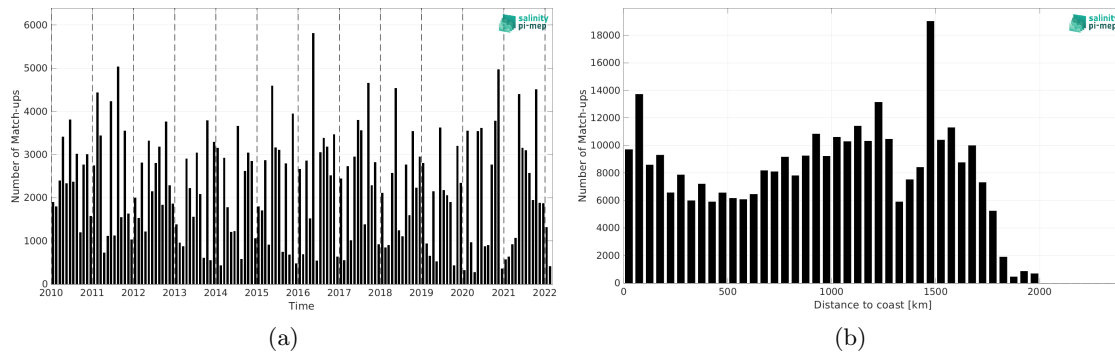
Figure 2: Number of match-ups between TSG (LEGOS-DM) and SMOS SSS L3 v335 - Monthly - 25 km (CATDS-CPDC) SSS as a function of time (a) and as function of the distance to coast (b) over the Amazon and Orinoco river plumes Pi-MEP region and for the full satellite product period.
