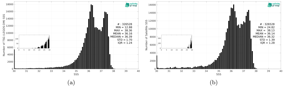
Figure 3: Histograms of SSS from TSG (LEGOS-DM) (a) and SMOS SSS L3 v335 - Monthly - 25 km (CATDS-CPDC) (b) considering all match-up pairs per bins of 0.1 over the Amazon and Orinoco river plumes Pi-MEP region and for the full satellite product period.
