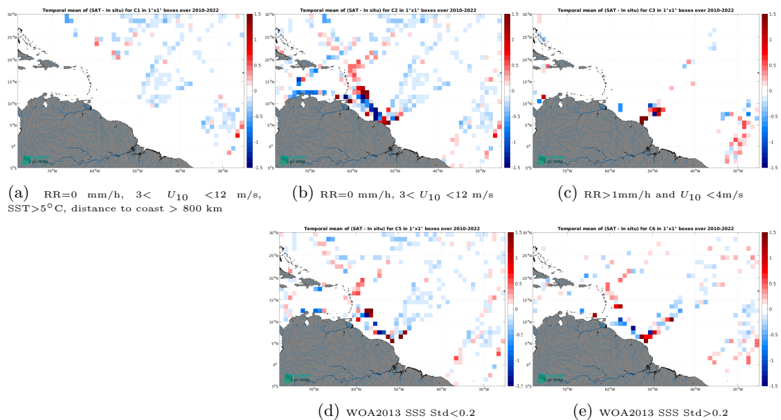
Figure 14: Temporal mean gridded over spatial boxes of size 1^\circ \times 1^\circ of \Delta\text{SSS} (SMOS SSS L3 v335 - Monthly - 25 km (CATDS-CPDC) - TSG (LEGOS-DM)) for 5 different subdatasets corresponding to:RR=0 mm/h, 3 < U_{10} < 12 m/s, SST >5^\circ\text{C} , distance to coast > 800 km (a), RR=0 mm/h, 3 < U_{10} < 12 m/s (b), RR >1 mm/h and U_{10} < 4 m/s (c), WOA2013 SSS Std <0.2 (d), WOA2013 SSS Std >0.2 (e).
