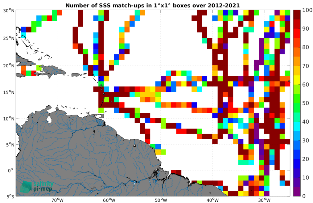
Figure 5: Number of SSS match-ups between TSG (GOSUD-Sailing-ship) SSS and the SMOS SSS L3 v335 - Monthly - 25 km (CATDS-CPDC) SSS product for the Amazon and Orinoco river plumes Pi-MEP region over 1^\circ \times 1^\circ boxes and for the full satellite product period.
