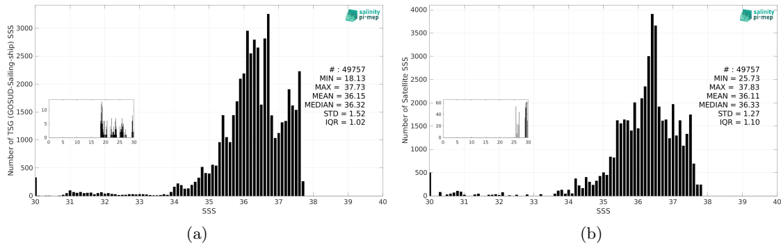
Figure 3: Histograms of SSS from TSG (GOSUD-Sailing-ship) (a) and SMOS SSS L3 v335 - Monthly - 25 km (CATDS-CPDC) (b) considering all match-up pairs per bins of 0.1 over the Amazon and Orinoco river plumes Pi-MEP region and for the full satellite product period.
