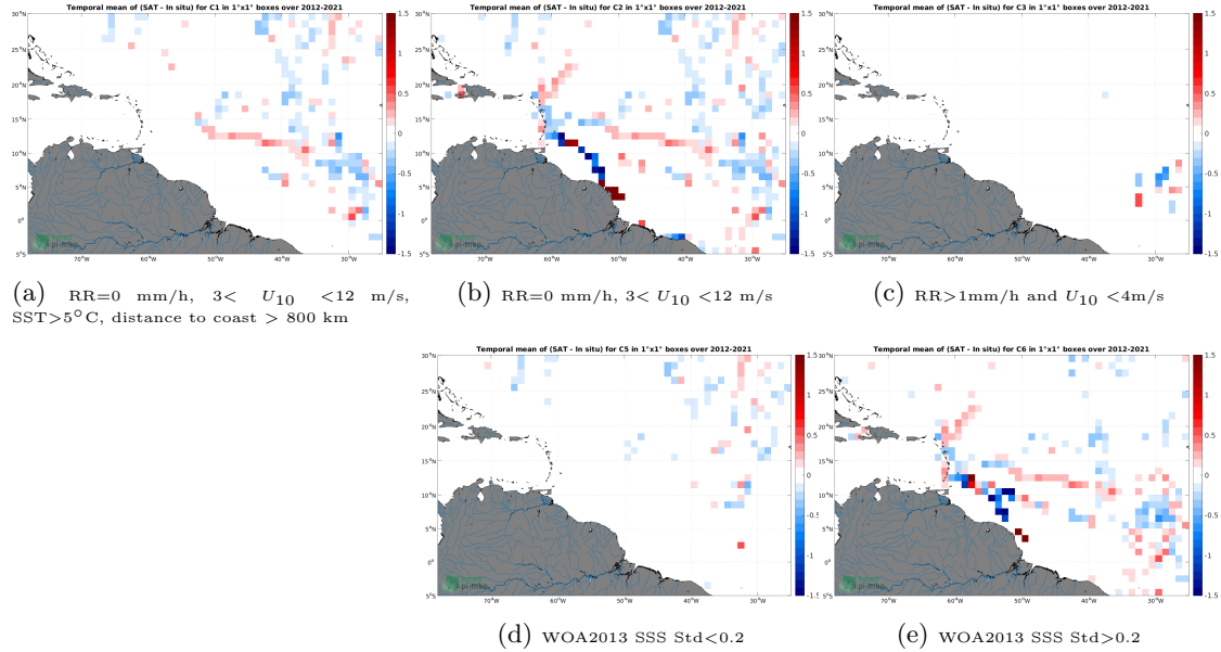
Figure 12: Temporal mean gridded over spatial boxes of size 1^{\circ}\times 1^{\circ} of \Delta SSS (SMOS SSS L3 v335 - Monthly - 25 km (CATDS-CPDC) - TSG (GOSUD-Sailing-ship)) for 5 different subdatasets corresponding to:RR=0 mm/h, 3 < U_{10} < 12 m/s, SST >5^{\circ}\text{C} , distance to coast > 800 km (a), RR=0 mm/h, 3 < U_{10} < 12 m/s (b), RR >1 mm/h and U_{10} < 4 m/s (c), WOA2013 SSS Std <0.2 (d), WOA2013 SSS Std >0.2 (e).
