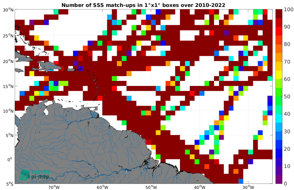
Figure 5: Number of SSS match-ups between TSG (GOSUD-Research-vessel) SSS and the SMOS SSS L3 v335 - Monthly - 25 km (CATDS-CPDC) SSS product for the Amazon and Orinoco river plumes Pi-MEP region over 1^\circ \times 1^\circ boxes and for the full satellite product period.
