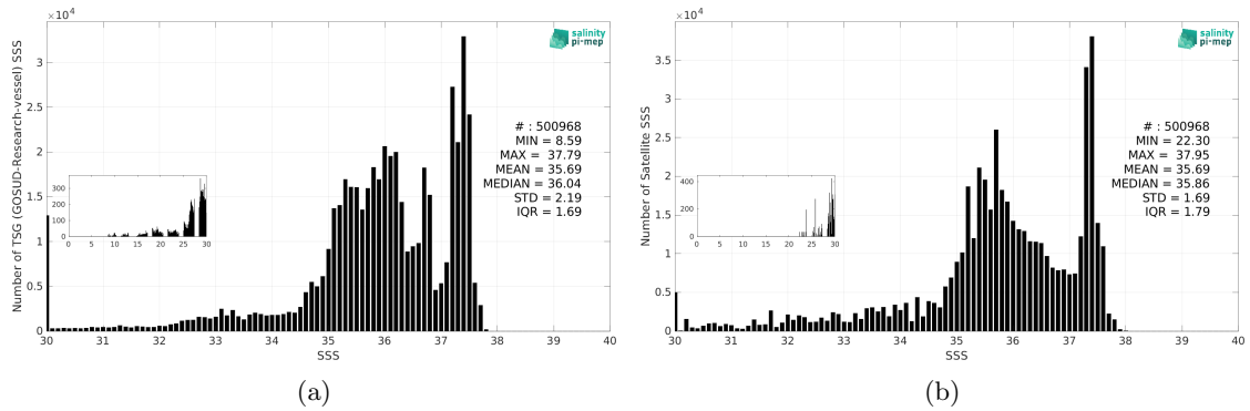
Figure 3: Histograms of SSS from TSG (GOSUD-Research-vessel) (a) and SMOS SSS L3 v335 - Monthly - 25 km (CATDS-CPDC) (b) considering all match-up pairs per bins of 0.1 over the Amazon and Orinoco river plumes Pi-MEP region and for the full satellite product period.
