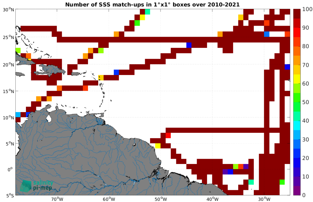
Figure 4: Number of SSS match-ups between TSG (CSIC-UTM) SSS and the SMOS SSS L3 v335 - Monthly - 25 km (CATDS-CPDC) SSS product for the Amazon and Orinoco river plumes Pi-MEP region over 1^\circ \times 1^\circ boxes and for the full satellite product period.
