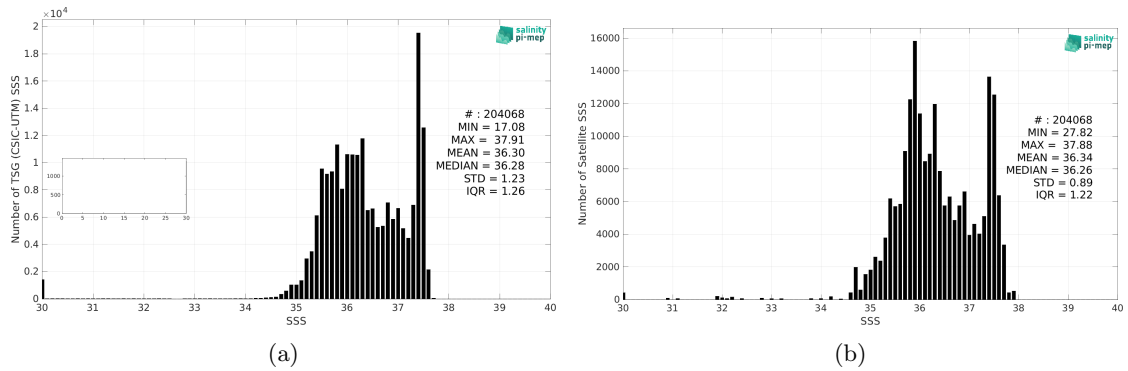
Figure 2: Histograms of SSS from TSG (CSIC-UTM) (a) and SMOS SSS L3 v335 - Monthly - 25 km (CATDS-CPDC) (b) considering all match-up pairs per bins of 0.1 over the Amazon and Orinoco river plumes Pi-MEP region and for the full satellite product period.
