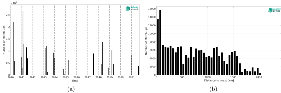
Figure 1: Number of match-ups between TSG (CSIC-UTM) and SMOS SSS L3 v335 - Monthly - 25 km (CATDS-CPDC) SSS as a function of time (a) and as function of the distance to coast (b) over the Amazon and Orinoco river plumes Pi-MEP region and for the full satellite product period.
