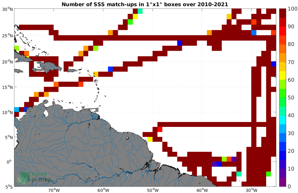
Figure 4: Number of SSS match-ups between TSG (CSIC-UTM) SSS and the SMOS SSS L3 v335 - Monthly - 25 km (CATDS-CPDC) SSS product for the Amazon and Orinoco river plumes Pi-MEP region over 1^{\circ} \times 1^{\circ} boxes and for the full satellite product period.
