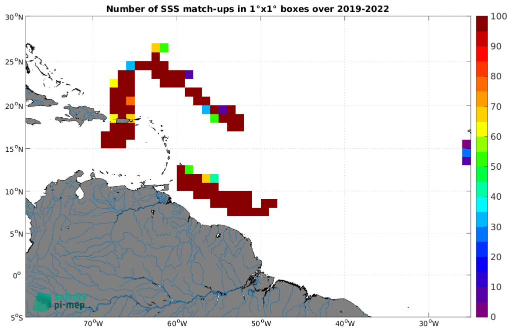
Figure 4: Number of SSS match-ups between Saildrone SSS and the SMOS SSS L3 v335 - Monthly - 25 km (CATDS-CPDC) SSS product for the Amazon and Orinoco river plumes Pi-MEP region over 1^\circ \times 1^\circ boxes and for the full satellite product period.
