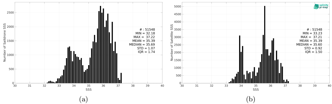
Figure 2: Histograms of SSS from Saildrone (a) and SMOS SSS L3 v335 - Monthly - 25 km (CATDS-CPDC) (b) considering all match-up pairs per bins of 0.1 over the Amazon and Orinoco river plumes Pi-MEP region and for the full satellite product period.
