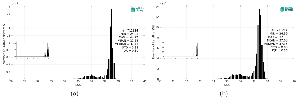
Figure 3: Histograms of SSS from Surface drifters (a) and SMOS SSS L3 v335 - Monthly - 25 km (CATDS-CPDC) (b) considering all match-up pairs per bins of 0.1 over the Amazon and Orinoco river plumes Pi-MEP region and for the full satellite product period.
