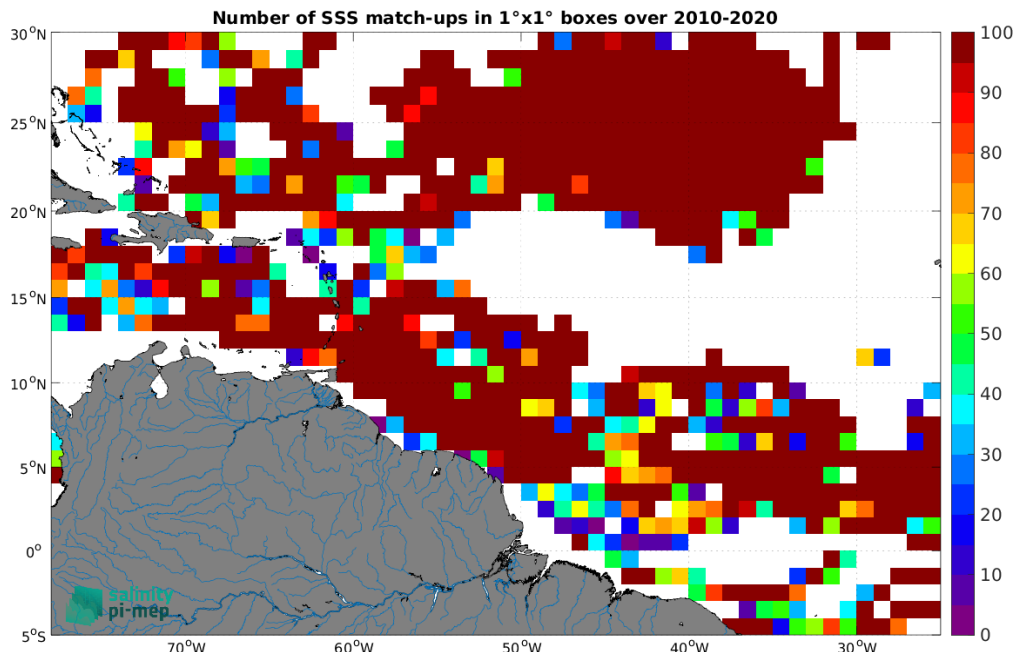
Figure 4: Number of SSS match-ups between Surface drifters SSS and the SMOS SSS L3 v335 - Monthly - 25 km (CATDS-CPDC) SSS product for the Amazon and Orinoco river plumes Pi-MEP region over 1^\circ \times 1^\circ boxes and for the full satellite product period.
