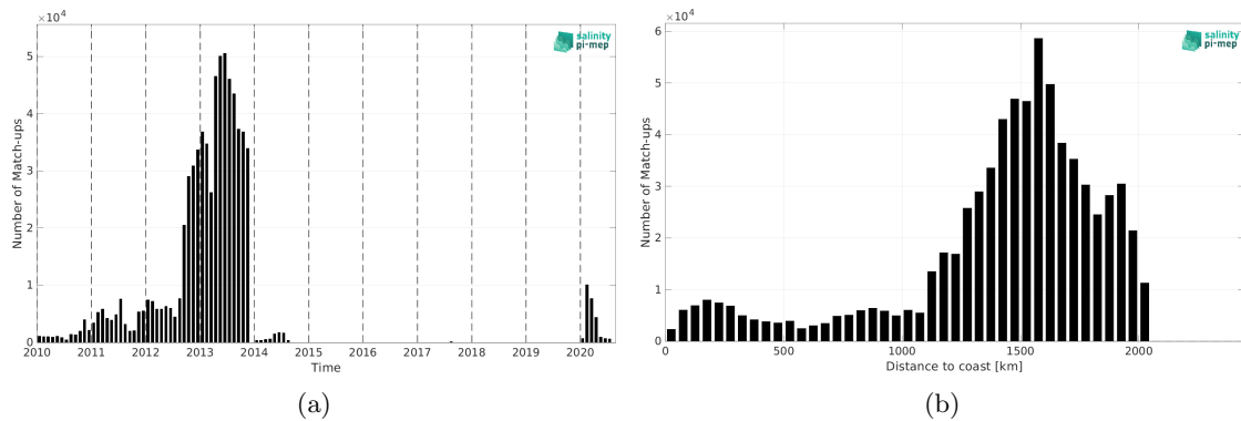
Figure 2: Number of match-ups between Surface drifters and SMOS SSS L3 v335 - Monthly - 25 km (CATDS-CPDC) SSS as a function of time (a) and as function of the distance to coast (b) over the Amazon and Orinoco river plumes Pi-MEP region and for the full satellite product period.
