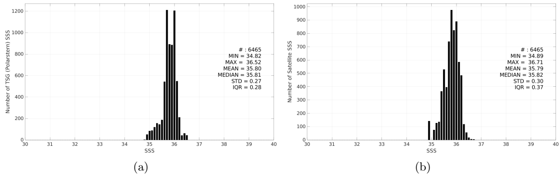
Figure 3: Histograms of SSS from TSG (Polarstern) (a) and SMOS SSS L3 v335 - 10 Days - 25 km (CATDS-CPDC) (b) considering all match-up pairs per bins of 0.1 over the Amazon and Orinoco river plumes Pi-MEP region and for the full satellite product period.
