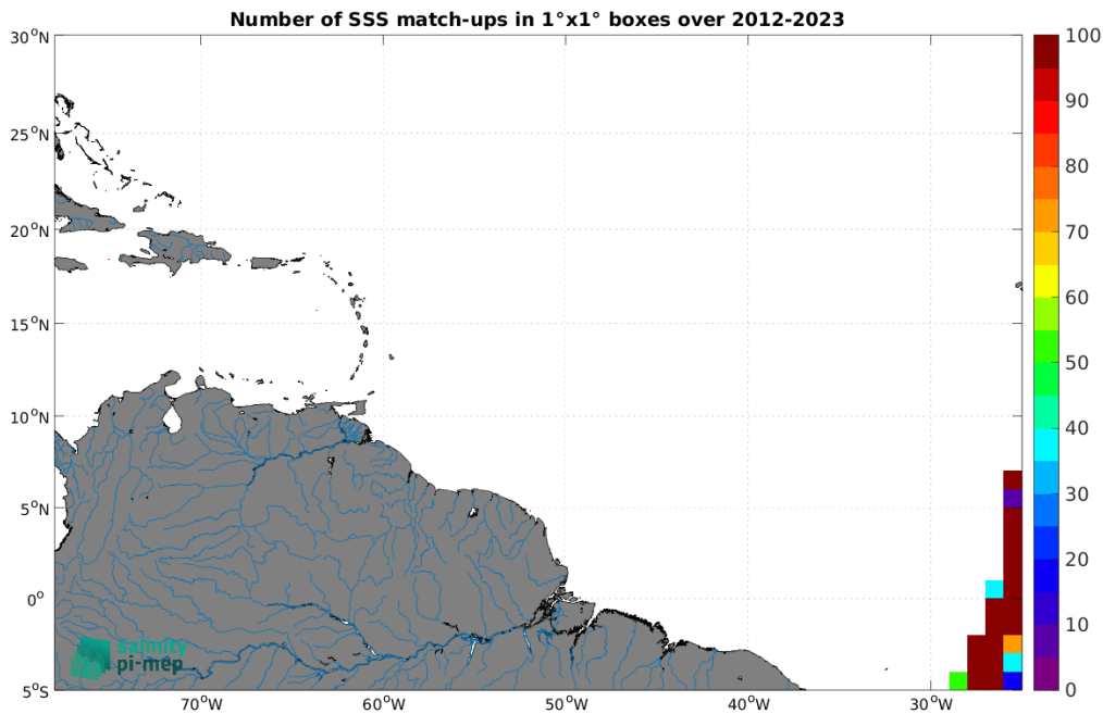
Figure 5: Number of SSS match-ups between TSG (Polarstern) SSS and the SMOS SSS L3 v335 - 10 Days - 25 km (CATDS-CPDC) SSS product for the Amazon and Orinoco river plumes Pi-MEP region over 1^\circ \times 1^\circ boxes and for the full satellite product period.
