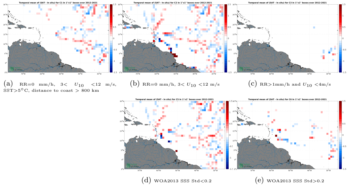
Figure 12: Temporal mean gridded over spatial boxes of size 1^{\circ}\times 1^{\circ} of \Delta SSS (SMOS SSS L3 v335 - 10 Days - 25 km (CATDS-CPDC) - TSG (GOSUD-Sailing-ship)) for 5 different subdatasets corresponding to:RR=0 mm/h, 3 < U_{10} < 12 m/s, SST >5^{\circ}\text{C} , distance to coast > 800 km (a), RR=0 mm/h, 3 < U_{10} < 12 m/s (b), RR >1 mm/h and U_{10} < 4 m/s (c), WOA2013 SSS Std <0.2 (d), WOA2013 SSS Std >0.2 (e).
