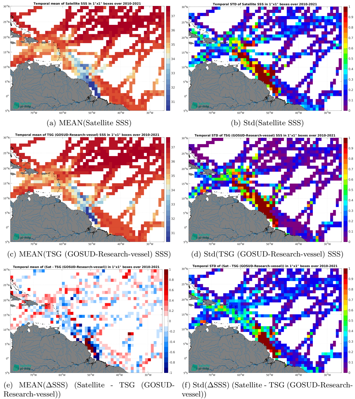
Figure 7: Temporal mean (left) and Std (right) of SSS from SMOS SSS L3 v335 - 10 Days - 25 km (CATDS-CPDC) (top), TSG (GOSUD-Research-vessel) (middle), and of \Delta SSS (Satellite - TSG (GOSUD-Research-vessel)). Only match-up pairs are used to generate these maps.
