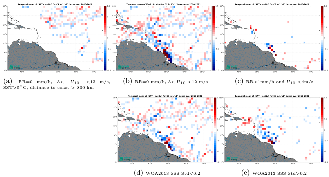
Figure 14: Temporal mean gridded over spatial boxes of size 1^\circ \times 1^\circ of \Delta\text{SSS} (SMOS SSS L3 v335 - 10 Days - 25 km (CATDS-CPDC) - TSG (GOSUD-Research-vessel)) for 5 different subdatasets corresponding to:RR=0 mm/h, 3 < U_{10} < 12 m/s, SST >5^\circ\text{C} , distance to coast > 800 km (a), RR=0 mm/h, 3 < U_{10} < 12 m/s (b), RR >1 mm/h and U_{10} < 4 m/s (c), WOA2013 SSS Std <0.2 (d), WOA2013 SSS Std >0.2 (e).
