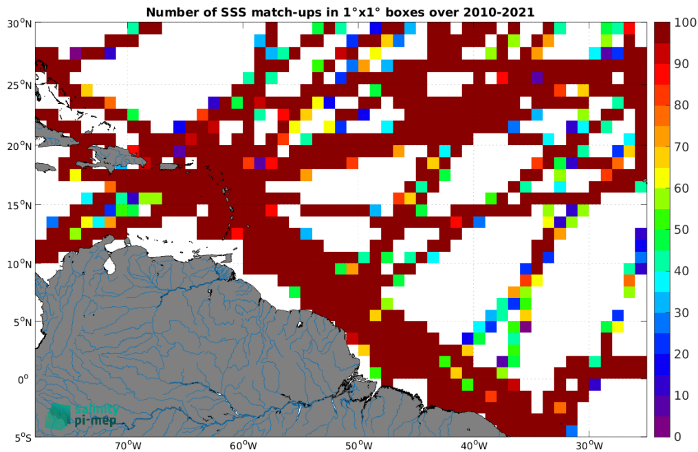
Figure 5: Number of SSS match-ups between TSG (GOSUD-Research-vessel) SSS and the SMOS SSS L3 v335 - 10 Days - 25 km (CATDS-CPDC) SSS product for the Amazon and Orinoco river plumes Pi-MEP region over 1^\circ \times 1^\circ boxes and for the full satellite product period.
