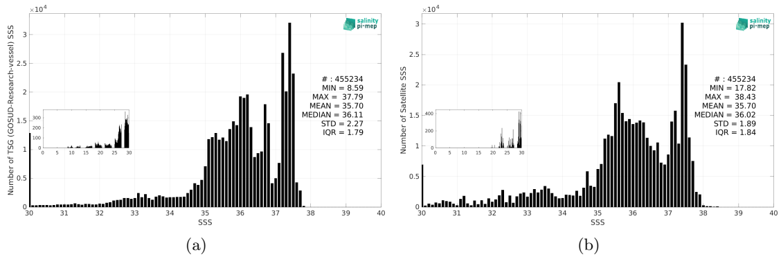
Figure 3: Histograms of SSS from TSG (GOSUD-Research-vessel) (a) and SMOS SSS L3 v335 - 10 Days - 25 km (CATDS-CPDC) (b) considering all match-up pairs per bins of 0.1 over the Amazon and Orinoco river plumes Pi-MEP region and for the full satellite product period.
