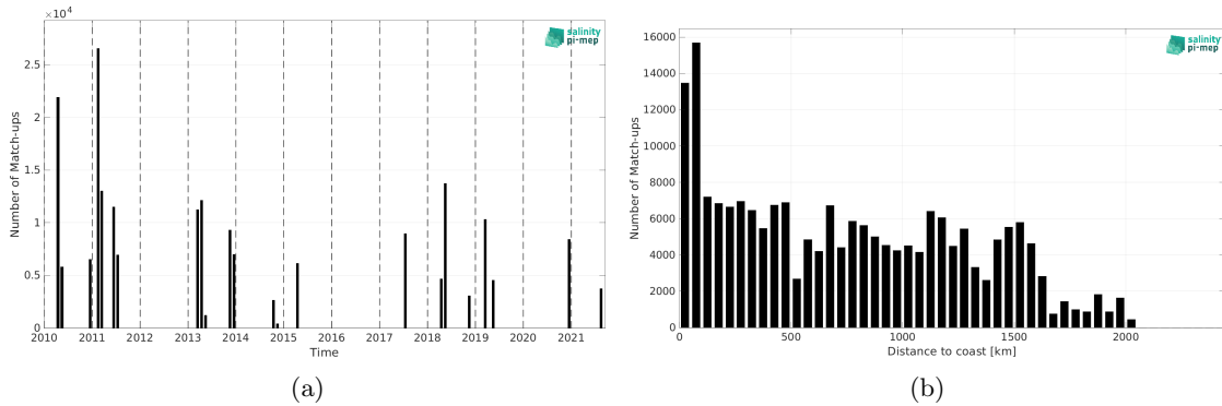
Figure 1: Number of match-ups between TSG (CSIC-UTM) and SMOS SSS L3 v335 - 10 Days - 25 km (CATDS-CPDC) SSS as a function of time (a) and as function of the distance to coast (b) over the Amazon and Orinoco river plumes Pi-MEP region and for the full satellite product period.
