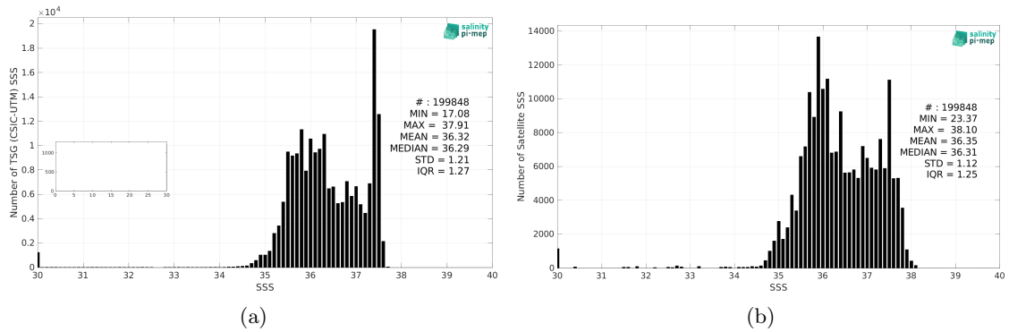
Figure 2: Histograms of SSS from TSG (CSIC-UTM) (a) and SMOS SSS L3 v335 - 10 Days - 25 km (CATDS-CPDC) (b) considering all match-up pairs per bins of 0.1 over the Amazon and Orinoco river plumes Pi-MEP region and for the full satellite product period.
