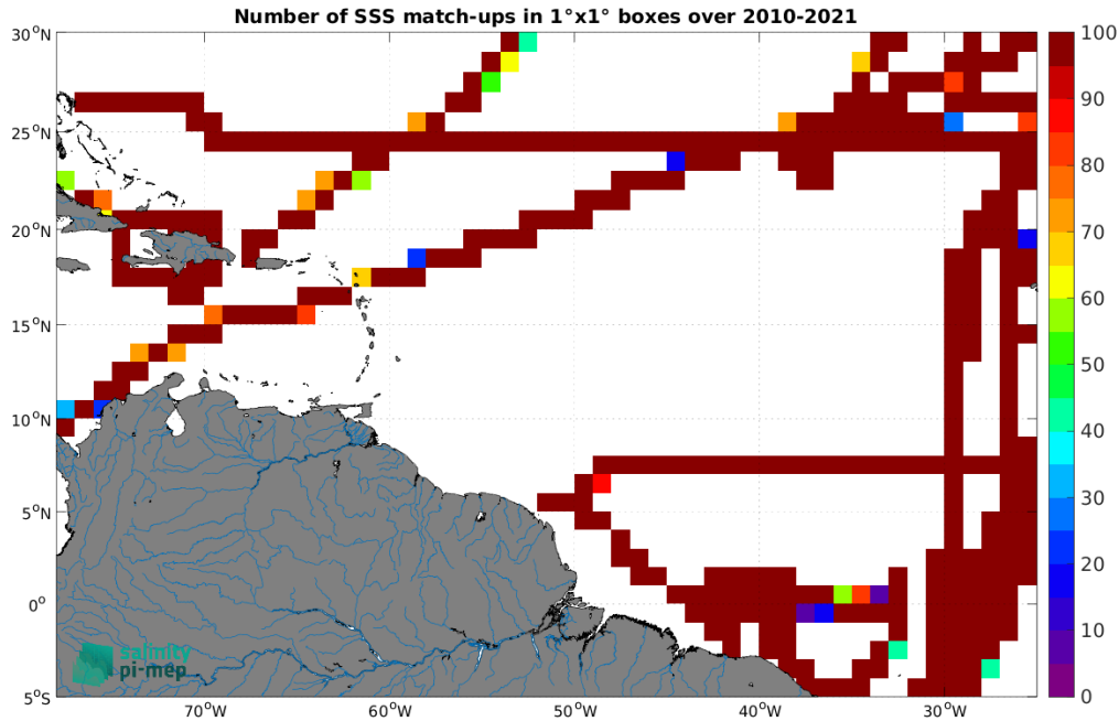
Figure 4: Number of SSS match-ups between TSG (CSIC-UTM) SSS and the SMOS SSS L3 v335 - 10 Days - 25 km (CATDS-CPDC) SSS product for the Amazon and Orinoco river plumes Pi-MEP region over 1^{\circ} \times 1^{\circ} boxes and for the full satellite product period.
