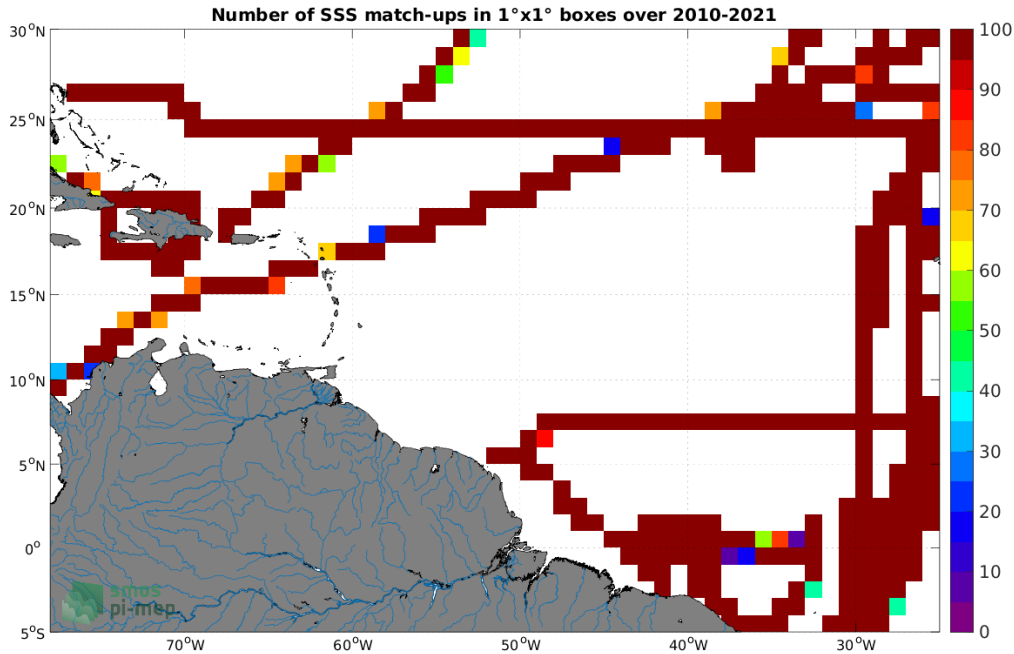
Figure 4: Number of SSS match-ups between TSG (CSIC-UTM) SSS and the SMOS SSS L3 v335 - 10 Days - 25 km (CATDS-CPDC) SSS product for the Amazon and Orinoco river plumes Pi-MEP region over 1^\circ \times 1^\circ boxes and for the full satellite product period.
