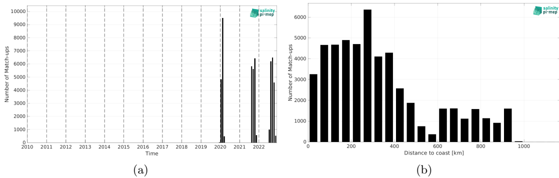
Figure 2: Number of match-ups between Saildrone and SMOS SSS L3 v335 - 10 Days - 25 km (CATDS-CPDC) SSS as a function of time (a) and as function of the distance to coast (b) over the Amazon and Orinoco river plumes Pi-MEP region and for the full satellite product period.
