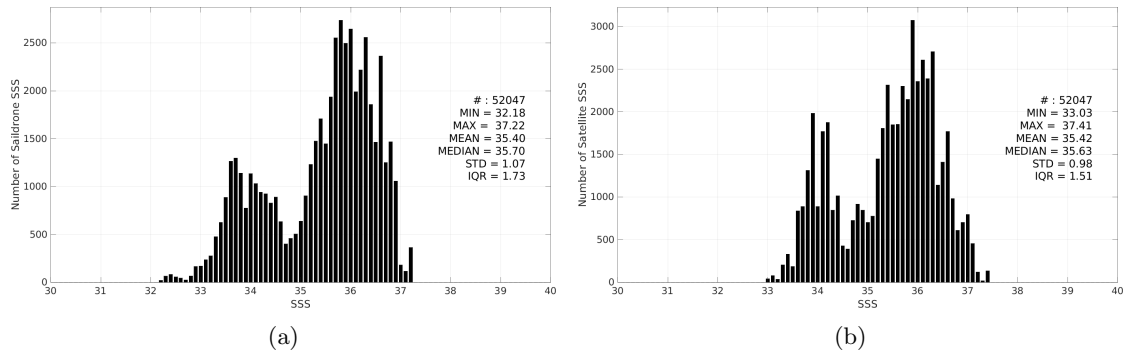
Figure 3: Histograms of SSS from Saildrone (a) and SMOS SSS L3 v335 - 10 Days - 25 km (CATDS-CPDC) (b) considering all match-up pairs per bins of 0.1 over the Amazon and Orinoco river plumes Pi-MEP region and for the full satellite product period.
