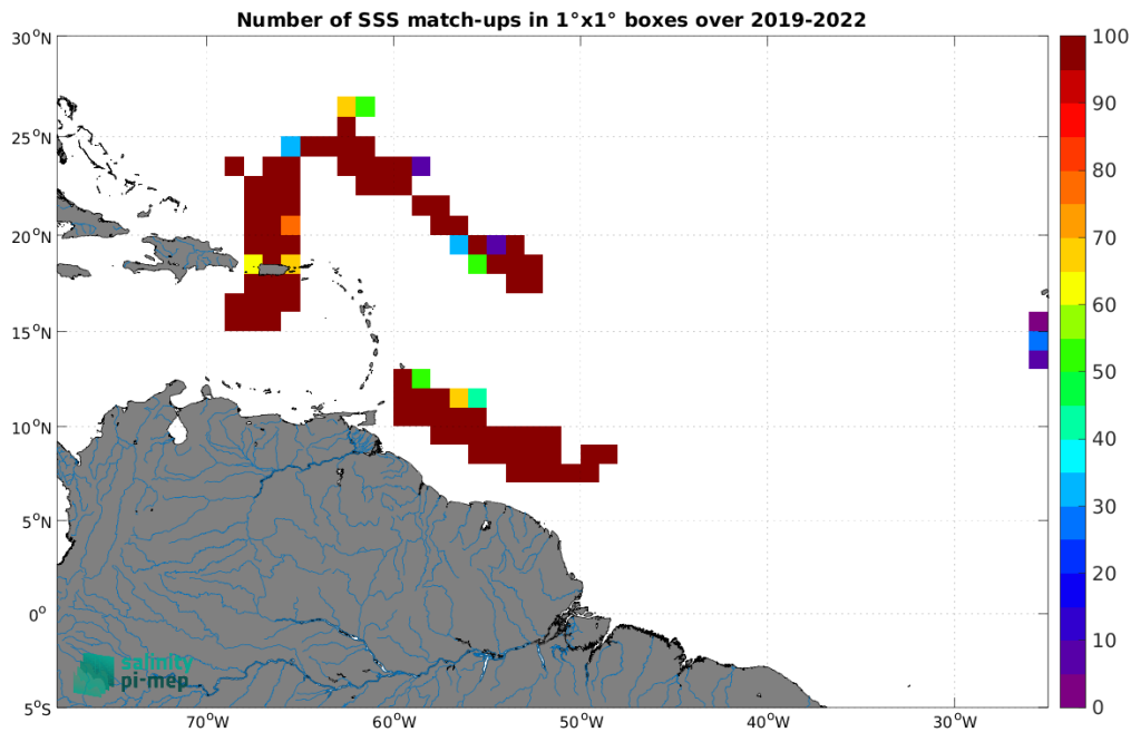
Figure 5: Number of SSS match-ups between Saildrone SSS and the SMOS SSS L3 v335 - 10 Days - 25 km (CATDS-CPDC) SSS product for the Amazon and Orinoco river plumes Pi-MEP region over 1^\circ \times 1^\circ boxes and for the full satellite product period.
