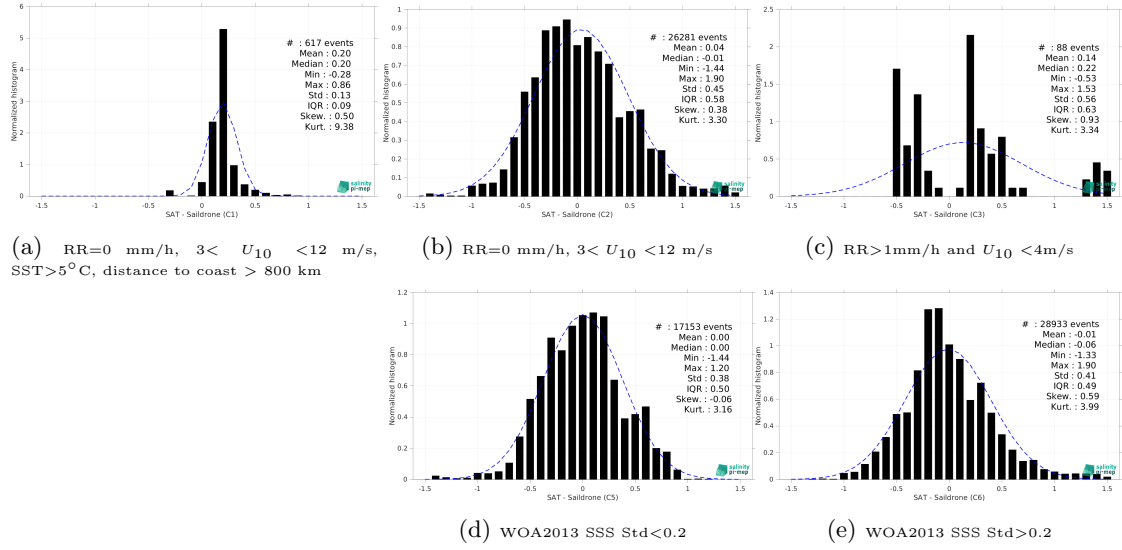
Figure 15: Normalized histogram of \Delta\text{SSS} (SMOS SSS L3 v335 - 10 Days - 25 km (CATDS-CPDC) - Sairdrone) for 5 different subdatasets corresponding to: RR=0 mm/h, 3 < U_{10} < 12 m/s, SST>5°C, distance to coast > 800 km (a), RR=0 mm/h, 3 < U_{10} < 12 m/s (b), RR>1mm/h and U_{10} < 4 m/s (c), WOA2013 SSS Std<0.2 (d), WOA2013 SSS Std>0.2 (e).
