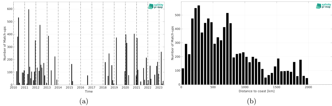
Figure 1: Number of match-ups between TSG (SAMOS) and SMOS SSS L2Q v331 - 0.25 Deg (CATDS-CPDC) SSS as a function of time (a) and as function of the distance to coast (b) over the Amazon and Orinoco river plumes Pi-MEP region and for the full satellite product period.
