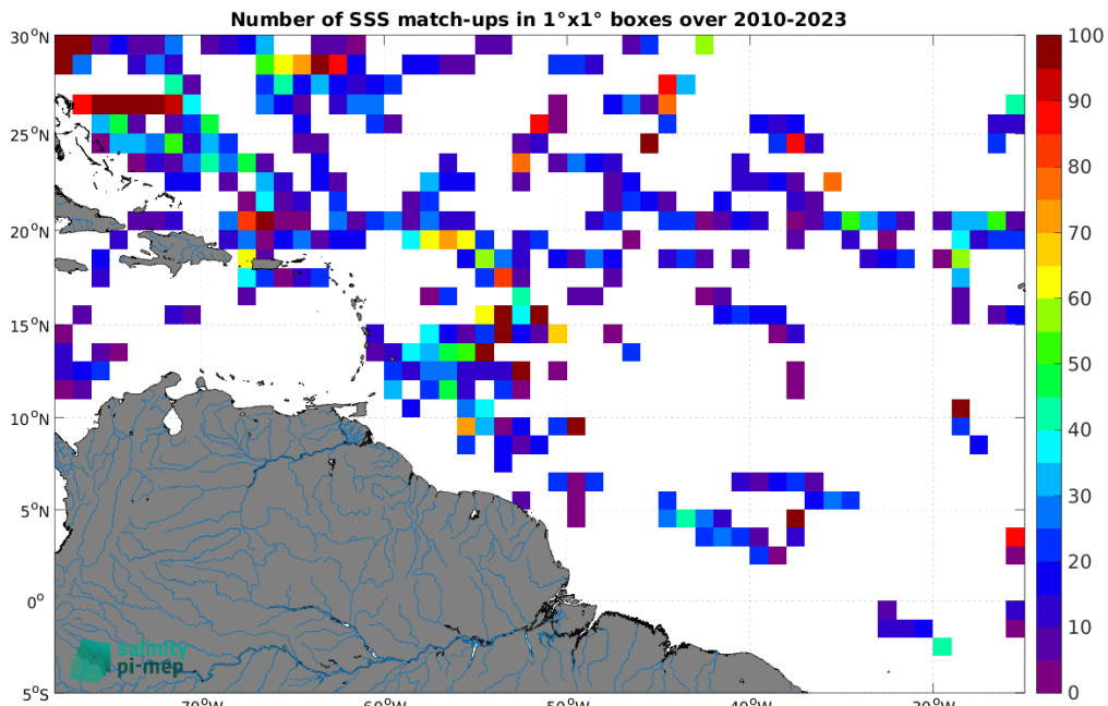
Figure 4: Number of SSS match-ups between TSG (SAMOS) SSS and the SMOS SSS L2Q v331 - 0.25 Deg (CATDS-CPDC) SSS product for the Amazon and Orinoco river plumes Pi-MEP region over 1^\circ \times 1^\circ boxes and for the full satellite product period.
