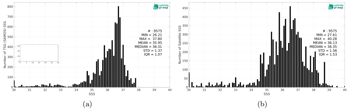
Figure 2: Histograms of SSS from TSG (SAMOS) (a) and SMOS SSS L2Q v331 - 0.25 Deg (CATDS-CPDC) (b) considering all match-up pairs per bins of 0.1 over the Amazon and Orinoco river plumes Pi-MEP region and for the full satellite product period.
