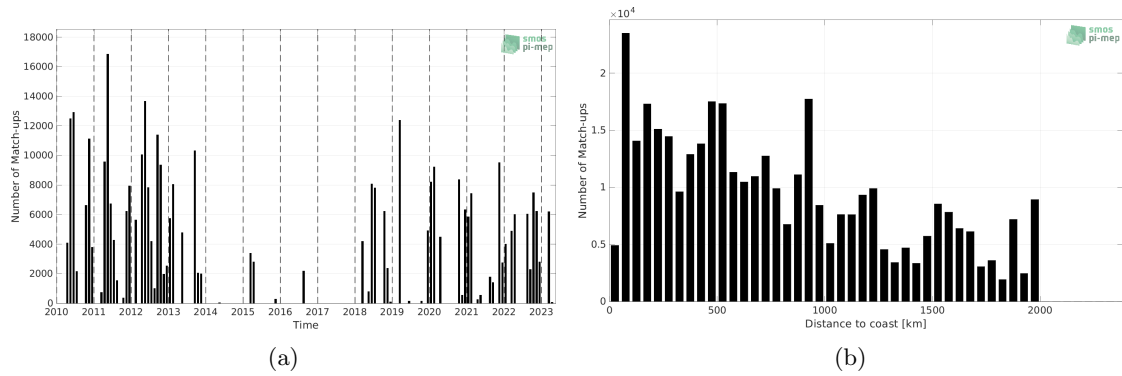
Figure 1: Number of match-ups between TSG (SAMOS) and SMOS SSS L2Q v331 - 0.25 Deg (CATDS-CPDC) SSS as a function of time (a) and as function of the distance to coast (b) over the Amazon and Orinoco river plumes Pi-MEP region and for the full satellite product period.
