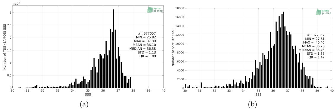
Figure 2: Histograms of SSS from TSG (SAMOS) (a) and SMOS SSS L2Q v331 - 0.25 Deg (CATDS-CPDC) (b) considering all match-up pairs per bins of 0.1 over the Amazon and Orinoco river plumes Pi-MEP region and for the full satellite product period.
