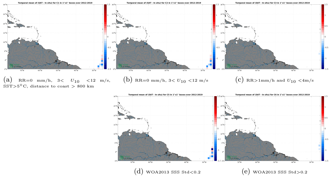
Figure 12: Temporal mean gridded over spatial boxes of size 1^\circ \times 1^\circ of \Delta SSS (SMOS SSS L2Q v331 - 0.25 Deg (CATDS-CPDC) - TSG (Polarstern)) for 5 different subdatasets corresponding to:RR=0 mm/h, 3 < U_{10} < 12 m/s, SST >5^\circ\text{C} , distance to coast > 800 km (a), RR=0 mm/h, 3 < U_{10} < 12 m/s (b), RR >1 mm/h and U_{10} < 4 m/s (c), WOA2013 SSS Std <0.2 (d), WOA2013 SSS Std >0.2 (e).
