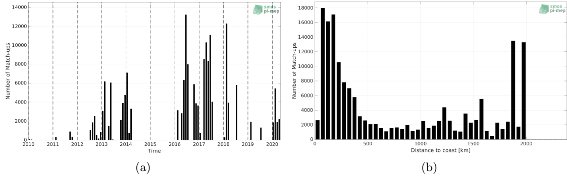
Figure 1: Number of match-ups between TSG (GOSUD-Research-vessel) and SMOS SSS L2Q v331 - 0.25 Deg (CATDS-CPDC) SSS as a function of time (a) and as function of the distance to coast (b) over the Amazon and Orinoco river plumes Pi-MEP region and for the full satellite product period.
