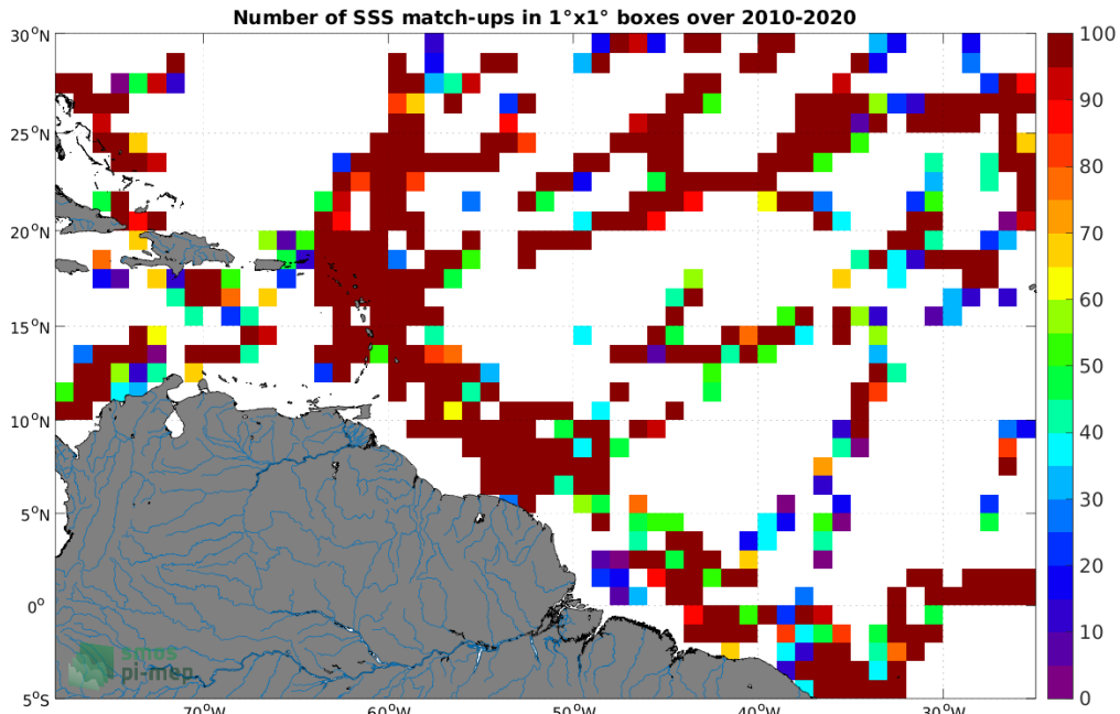
Figure 4: Number of SSS match-ups between TSG (GOSUD-Research-vessel) SSS and the SMOS SSS L2Q v331 - 0.25 Deg (CATDS-CPDC) SSS product for the Amazon and Orinoco river plumes Pi-MEP region over 1^\circ \times 1^\circ boxes and for the full satellite product period.
