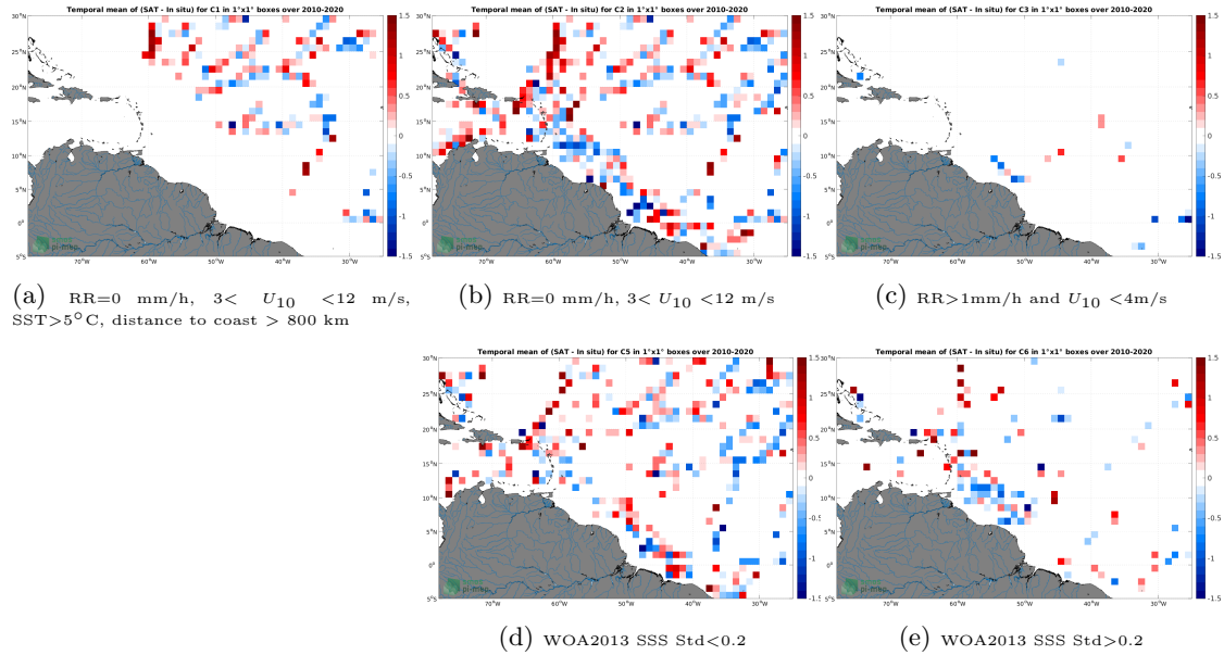
Figure 12: Temporal mean gridded over spatial boxes of size 1^\circ \times 1^\circ of \Delta SSS (SMOS SSS L2Q v331 - 0.25 Deg (CATDS-CPDC) - TSG (GOSUD-Research-vessel)) for 5 different subdatasets corresponding to:RR=0 mm/h, 3 < U_{10} < 12 m/s, SST >5^\circ\text{C} , distance to coast > 800 km (a), RR=0 mm/h, 3 < U_{10} < 12 m/s (b), RR >1 mm/h and U_{10} < 4 m/s (c), WOA2013 SSS Std <0.2 (d), WOA2013 SSS Std >0.2 (e).
