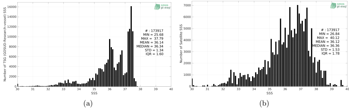
Figure 2: Histograms of SSS from TSG (GOSUD-Research-vessel) (a) and SMOS SSS L2Q v331 - 0.25 Deg (CATDS-CPDC) (b) considering all match-up pairs per bins of 0.1 over the Amazon and Orinoco river plumes Pi-MEP region and for the full satellite product period.
