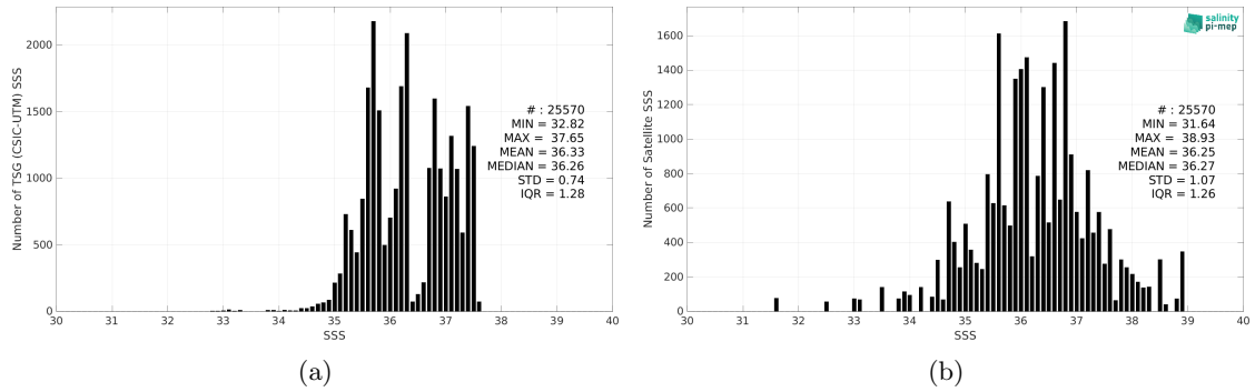
Figure 2: Histograms of SSS from TSG (CSIC-UTM) (a) and SMOS SSS L2Q v331 - 0.25 Deg (CATDS-CPDC) (b) considering all match-up pairs per bins of 0.1 over the Amazon and Orinoco river plumes Pi-MEP region and for the full satellite product period.
