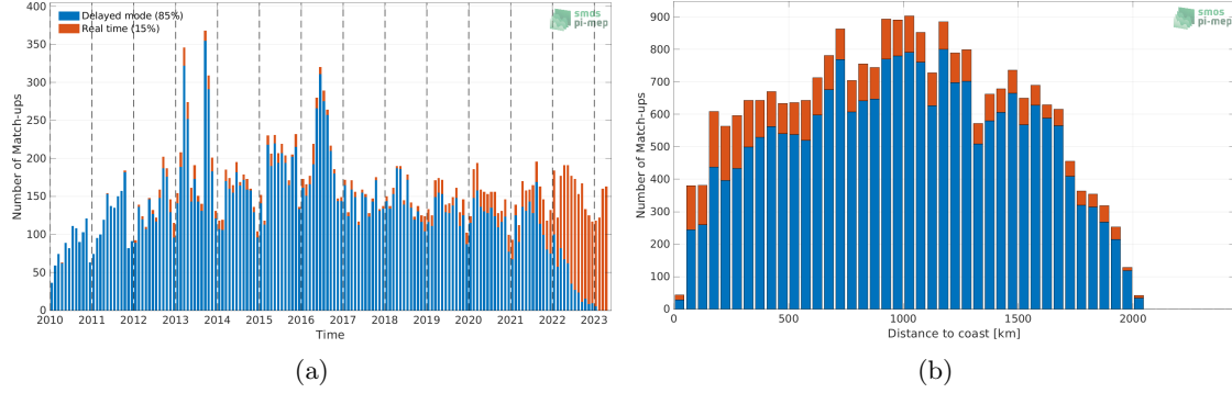
Figure 1: Number of match-ups between Argo and SMOS SSS L2Q v331 - 0.25 Deg (CATDS-CPDC) SSS as a function of time (a) and as function of the distance to coast (b) over the Amazon and Orinoco river plumes Pi-MEP region and for the full satellite product period.
