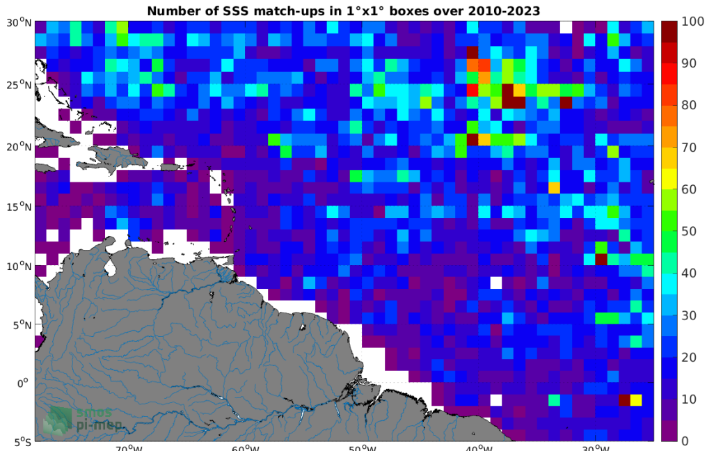
Figure 4: Number of SSS match-ups between Argo SSS and the SMOS SSS L2Q v331 - 0.25 Deg (CATDS-CPDC) SSS product for the Amazon and Orinoco river plumes Pi-MEP region over 1^\circ \times 1^\circ boxes and for the full satellite product period.
