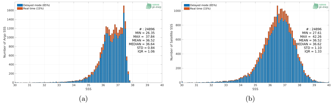
Figure 2: Histograms of SSS from Argo (a) and SMOS SSS L2Q v331 - 0.25 Deg (CATDS-CPDC) (b) considering all match-up pairs per bins of 0.1 over the Amazon and Orinoco river plumes Pi-MEP region and for the full satellite product period.
