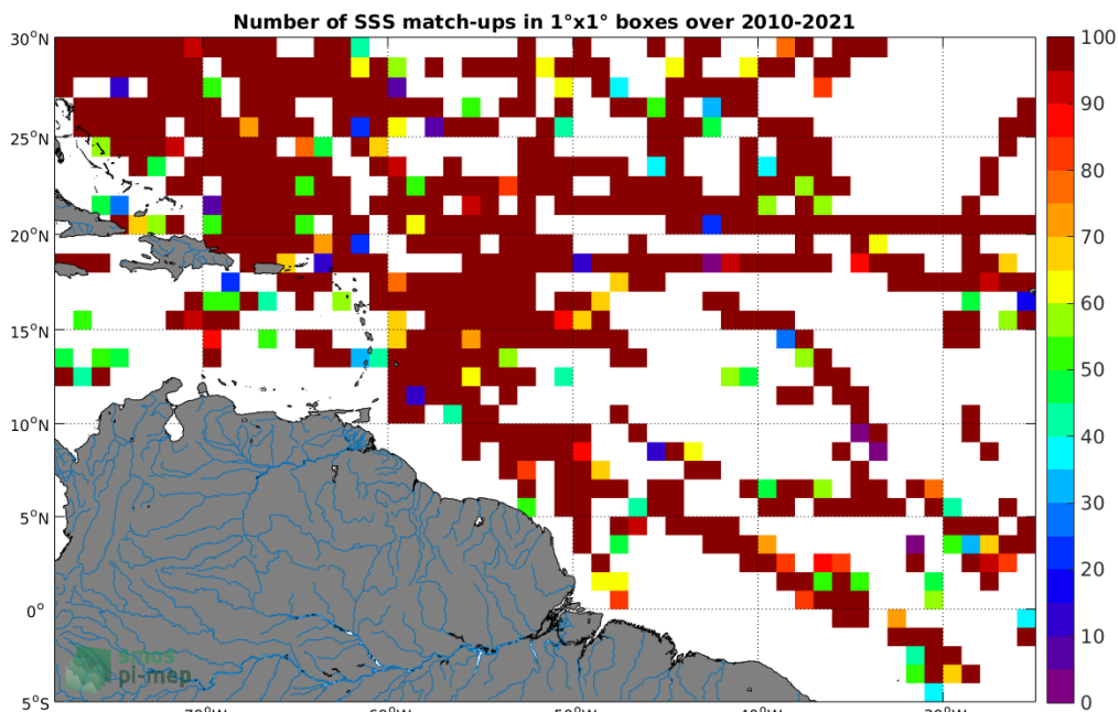
Figure 4: Number of SSS match-ups between TSG (SAMOS) SSS and the SMOS SSS L2Q v321 - 0.25 Deg (CATDS-CPDC) SSS product for the Amazon and Orinoco river plumes Pi-MEP region over 1^\circ \times 1^\circ boxes and for the full satellite product period.
