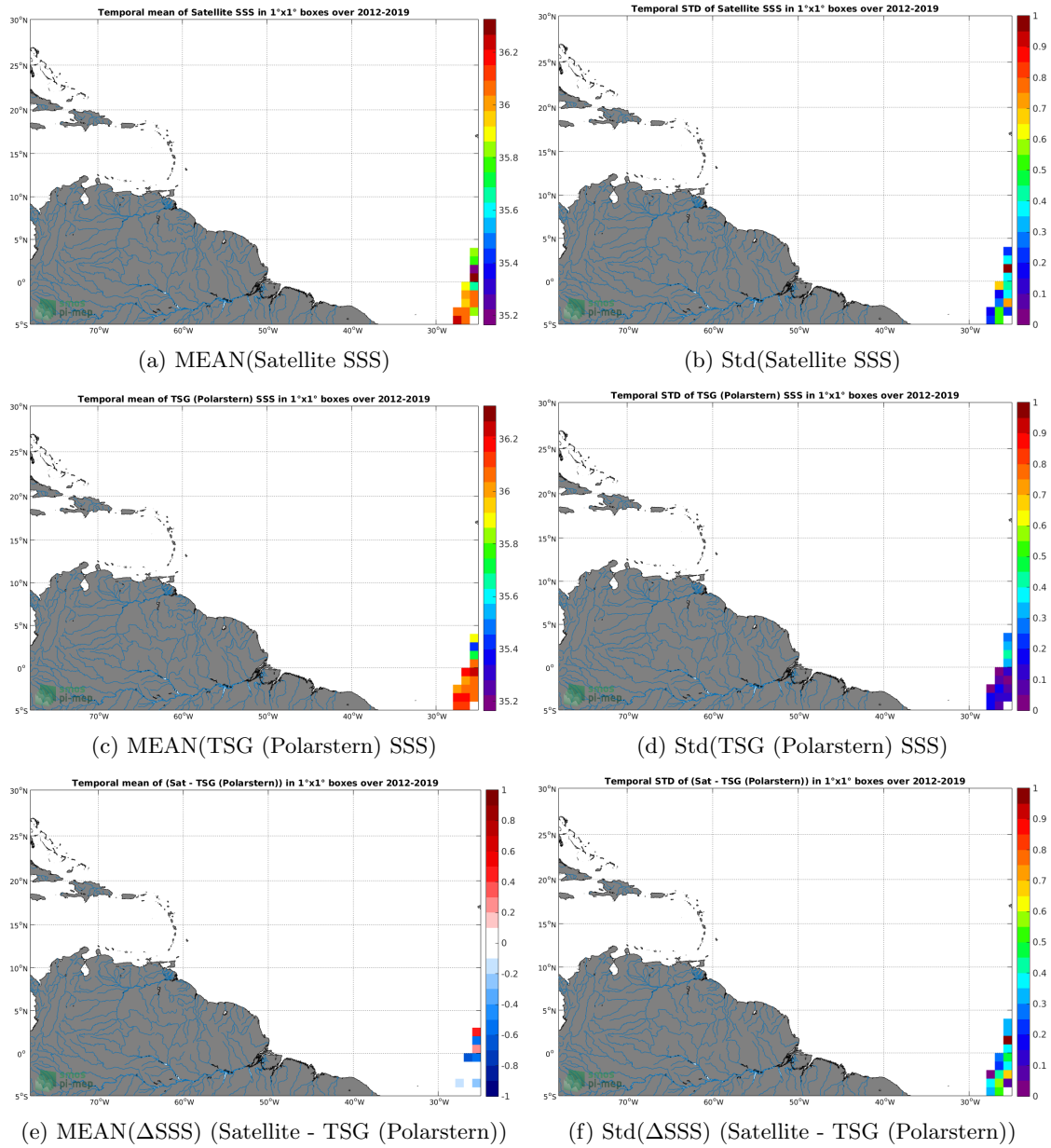
Figure 6: Temporal mean (left) and Std (right) of SSS from SMOS SSS L2Q v321 - 0.25 Deg (CATDS-CPDC) (top), TSG (Polarstern) (middle), and of \Delta SSS (Satellite - TSG (Polarstern)). Only match-up pairs are used to generate these maps.
