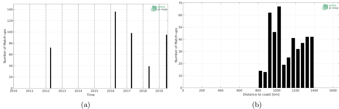
Figure 1: Number of match-ups between TSG (Polarstern) and SMOS SSS L2Q v321 - 0.25 Deg (CATDS-CPDC) SSS as a function of time (a) and as function of the distance to coast (b) over the Amazon and Orinoco river plumes Pi-MEP region and for the full satellite product period.
