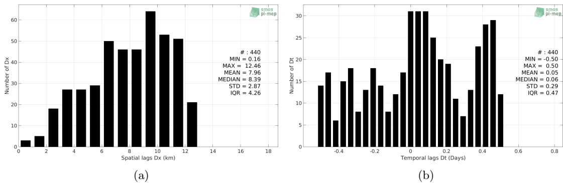
Figure 5: Histograms of the spatial (a) and temporal (b) lags between the location/time of the TSG (Polarstern) measurement and the date of the corresponding SMOS SSS L2Q v321 - 0.25 Deg (CATDS-CPDC) SSS pixel.
