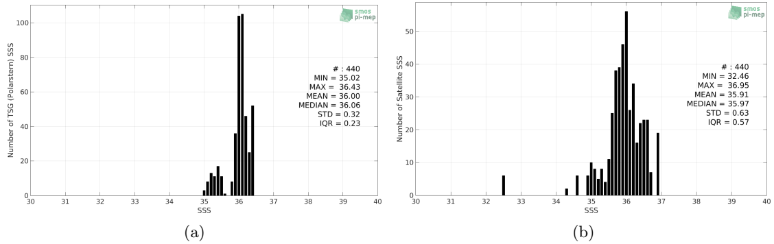
Figure 2: Histograms of SSS from TSG (Polarstern) (a) and SMOS SSS L2Q v321 - 0.25 Deg (CATDS-CPDC) (b) considering all match-up pairs per bins of 0.1 over the Amazon and Orinoco river plumes Pi-MEP region and for the full satellite product period.
