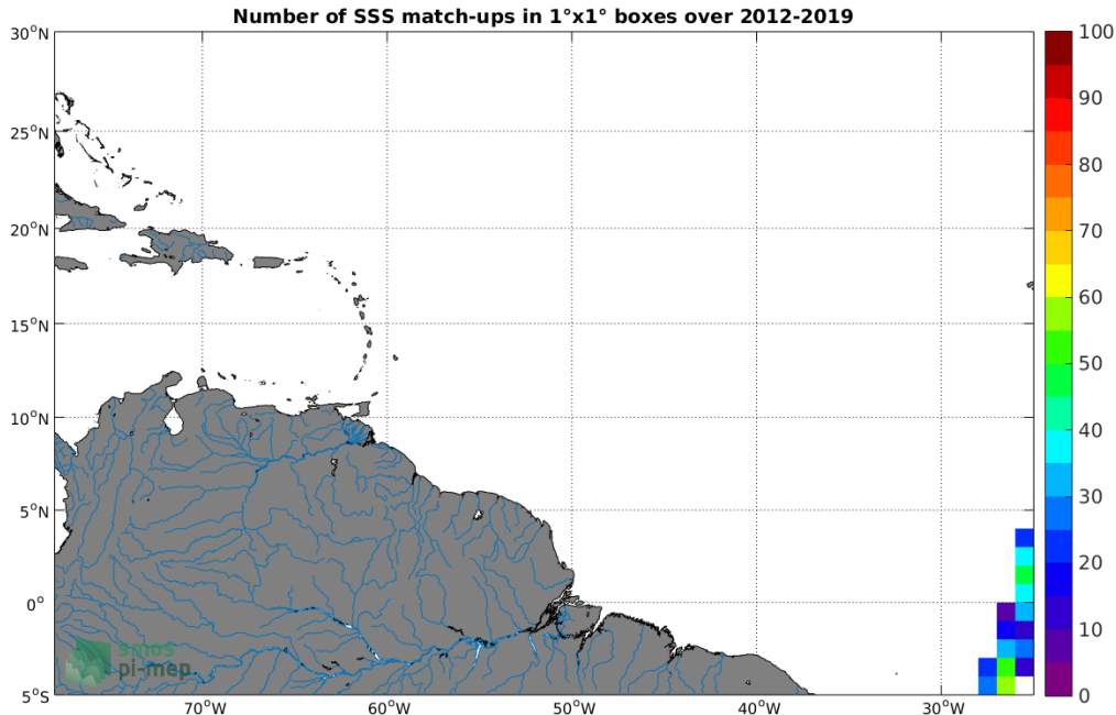
Figure 4: Number of SSS match-ups between TSG (Polarstern) SSS and the SMOS SSS L2Q v321 - 0.25 Deg (CATDS-CPDC) SSS product for the Amazon and Orinoco river plumes Pi-MEP region over 1°x1° boxes and for the full satellite product period.
