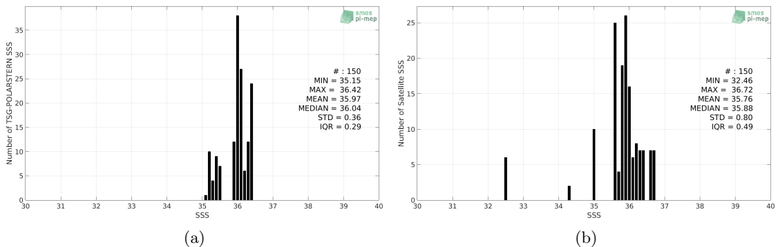
Figure 2: Histograms of SSS from TSG-POLARSTERN (a) and SMOS-L3-CATDS-CPDC-V321-L2Q (b) considering all match-up pairs per bins of 0.1 over the Amazon and Orinoco river plumes Pi-MEP region and for the full satellite product period.
