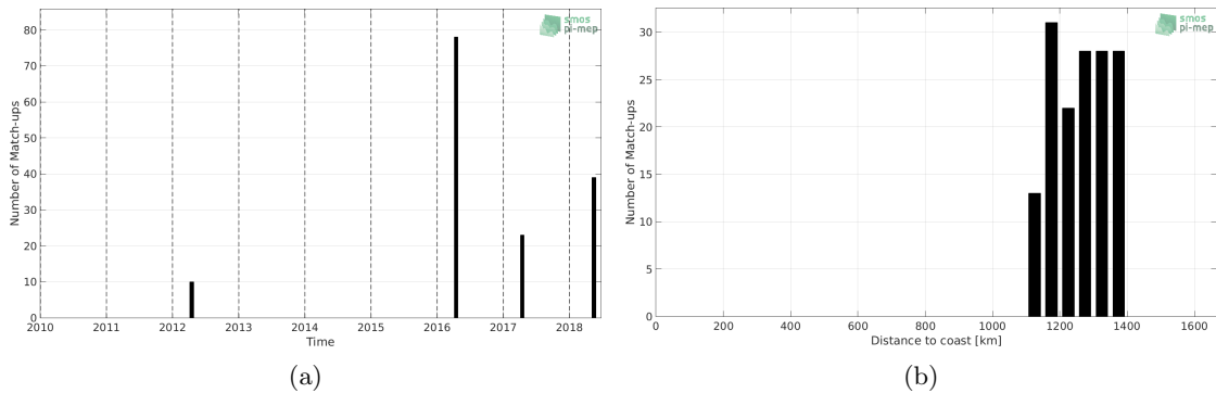
Figure 1: Number of match-ups between TSG-POLARSTERN and SMOS-L3-CATDS-CPDC-V321-L2Q SSS as a function of time (a) and as function of the distance to coast (b) over the Amazon and Orinoco river plumes Pi-MEP region and for the full satellite product period.
