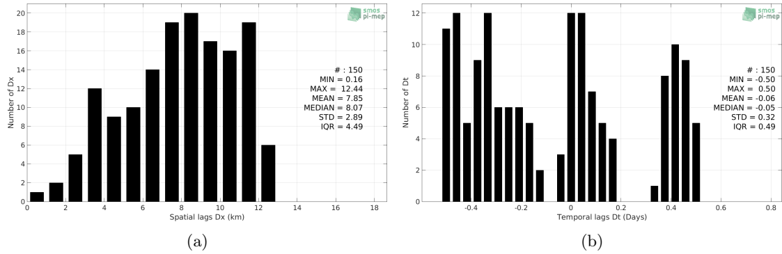
Figure 5: Histograms of the spatial (a) and temporal (b) lags between the time of the TSG-POLARSTERN measurements and the date of the corresponding SMOS-L3-CATDS-CPDC-V321-L2Q SSS product.
