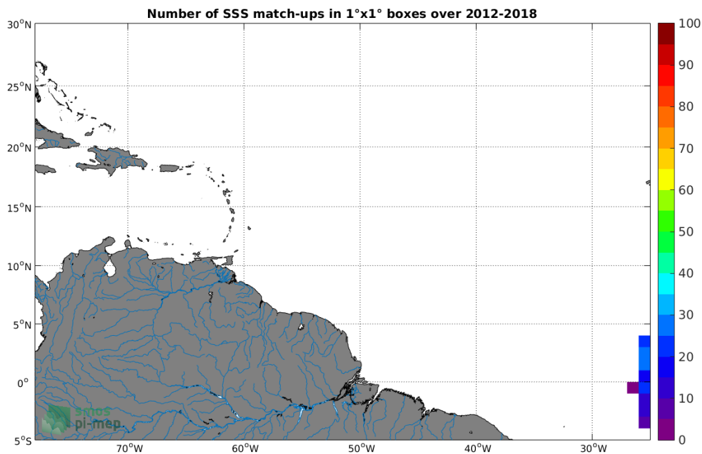
Figure 4: Number of SSS match-ups between TSG-POLARSTERN SSS and the SMOS-L3-CATDS-CPDC-V321-L2Q SSS product for the Amazon and Orinoco river plumes Pi-MEP region over 1^\circ \times 1^\circ boxes and for the full satellite product period.
