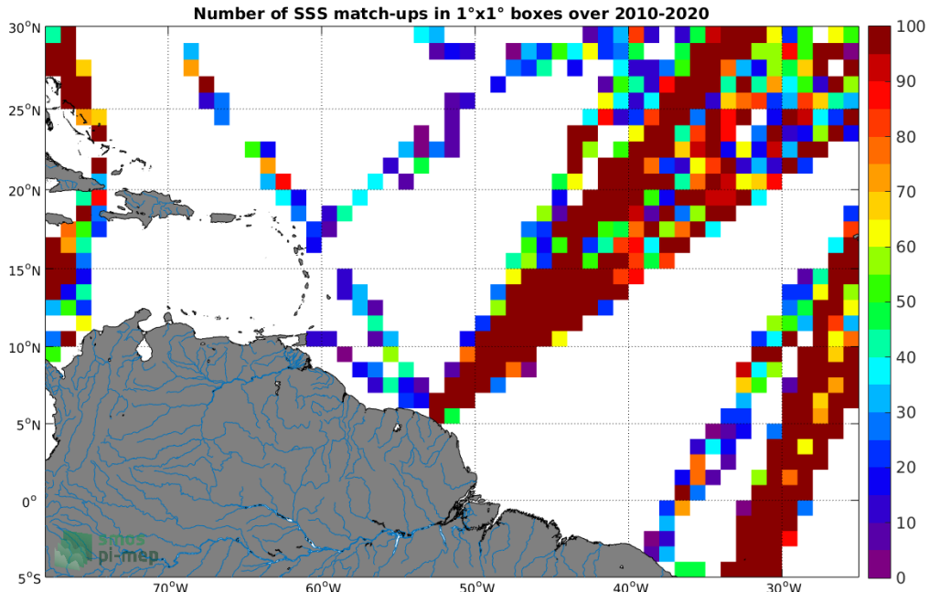
Figure 4: Number of SSS match-ups between TSG (LEGOS-DM) SSS and the SMOS SSS L2Q v321 - 0.25 Deg (CATDS-CPDC) SSS product for the Amazon and Orinoco river plumes Pi-MEP region over 1^\circ \times 1^\circ boxes and for the full satellite product period.
