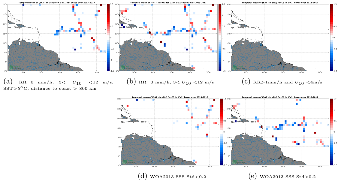
Figure 12: Temporal mean gridded over spatial boxes of size 1^\circ \times 1^\circ of \Delta SSS (SMOS SSS L2Q v321 - 0.25 Deg (CATDS-CPDC) - TSG (GOSUD-Sailing-ship)) for 5 different subdatasets corresponding to: RR=0 mm/h, 3 < U_{10} < 12 m/s, SST >5^\circ\text{C} , distance to coast > 800 km (a), RR=0 mm/h, 3 < U_{10} < 12 m/s (b), RR >1 mm/h and U_{10} < 4 m/s (c), WOA2013 SSS Std <0.2 (d), WOA2013 SSS Std >0.2 (e).
