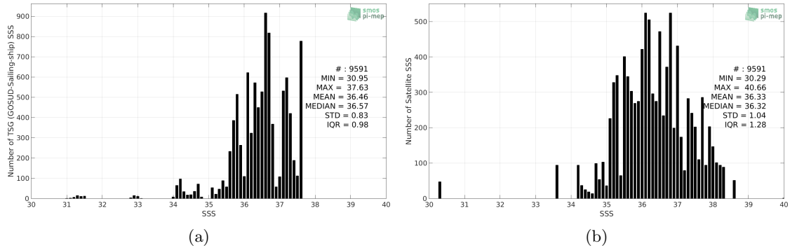
Figure 2: Histograms of SSS from TSG (GOSUD-Sailing-ship) (a) and SMOS SSS L2Q v321 - 0.25 Deg (CATDS-CPDC) (b) considering all match-up pairs per bins of 0.1 over the Amazon and Orinoco river plumes Pi-MEP region and for the full satellite product period.
