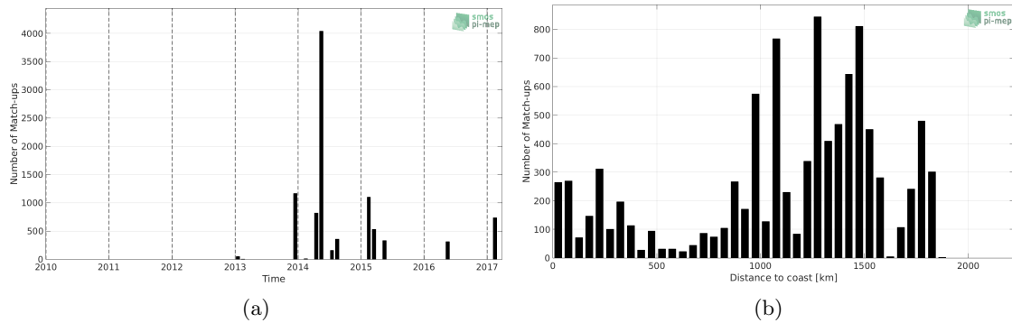
Figure 1: Number of match-ups between TSG (GOSUD-Sailing-ship) and SMOS SSS L2Q v321 - 0.25 Deg (CATDS-CPDC) SSS as a function of time (a) and as function of the distance to coast (b) over the Amazon and Orinoco river plumes Pi-MEP region and for the full satellite product period.
