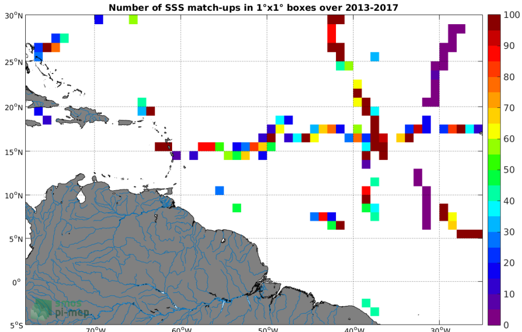
Figure 4: Number of SSS match-ups between TSG (GOSUD-Sailing-ship) SSS and the SMOS SSS L2Q v321 - 0.25 Deg (CATDS-CPDC) SSS product for the Amazon and Orinoco river plumes Pi-MEP region over 1^{\circ} \times 1^{\circ} boxes and for the full satellite product period.
