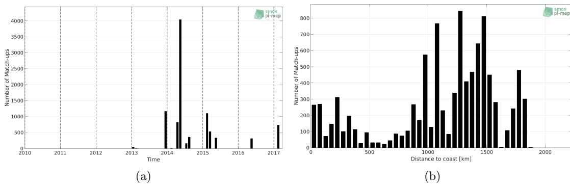
Figure 1: Number of match-ups between TSG (GOSUD-Sailing-ship) and SMOS SSS L2Q v321 - 0.25 Deg (CATDS-CPDC) SSS as a function of time (a) and as function of the distance to coast (b) over the Amazon and Orinoco river plumes Pi-MEP region and for the full satellite product period.
