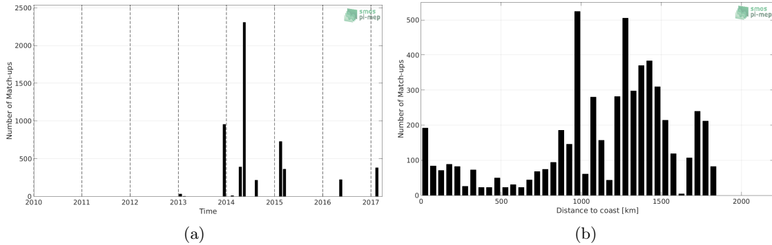
Figure 1: Number of match-ups between TSG-GOSUD-Sailing-ship and SMOS-L3-CATDS-CPDC-V321-L2Q SSS as a function of time (a) and as function of the distance to coast (b) over the Amazon and Orinoco river plumes Pi-MEP region and for the full satellite product period.
