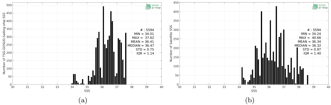
Figure 2: Histograms of SSS from TSG-GOSUD-Sailing-ship (a) and SMOS-L3-CATDS-CPDC-V321-L2Q (b) considering all match-up pairs per bins of 0.1 over the Amazon and Orinoco river plumes Pi-MEP region and for the full satellite product period.
