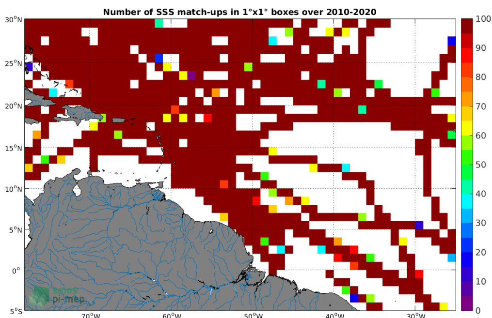
Figure 4: Number of SSS match-ups between TSG-SAMOS SSS and the SMOS L3 v317 - Monthly - 25 km (CATDS-CPDC) SSS product for the Amazon and Orinoco river plumes Pi-MEP region over 1°x1° boxes and for the full satellite product period.
