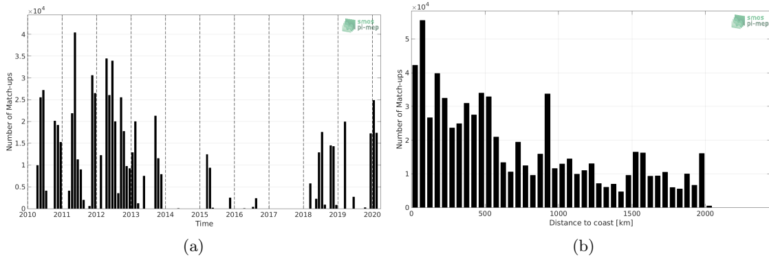
Figure 1: Number of match-ups between TSG-SAMOS and SMOS L3 v317 - Monthly - 25 km (CATDS-CPDC) SSS as a function of time (a) and as function of the distance to coast (b) over the Amazon and Orinoco river plumes Pi-MEP region and for the full satellite product period.
