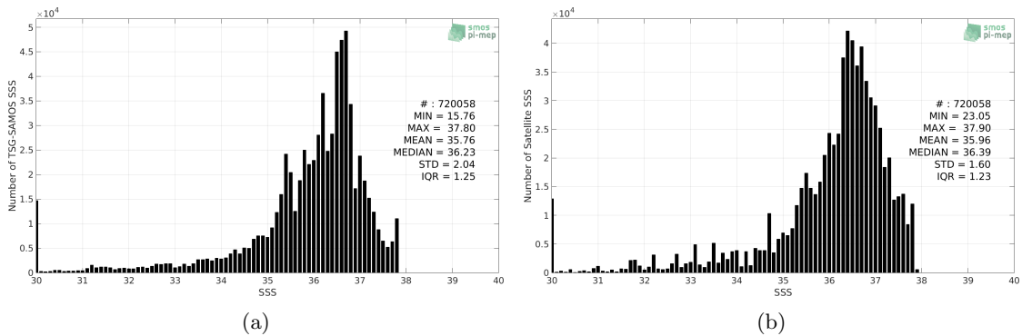
Figure 2: Histograms of SSS from TSG-SAMOS (a) and SMOS L3 v317 - Monthly - 25 km (CATDS-CPDC) (b) considering all match-up pairs per bins of 0.1 over the Amazon and Orinoco river plumes Pi-MEP region and for the full satellite product period.
