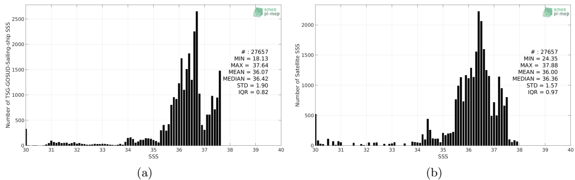
Figure 2: Histograms of SSS from TSG-GOSUD-Sailing-ship (a) and SMOS L3 v317 - Monthly - 25 km (CATDS-CPDC) (b) considering all match-up pairs per bins of 0.1 over the Amazon and Orinoco river plumes Pi-MEP region and for the full satellite product period.
