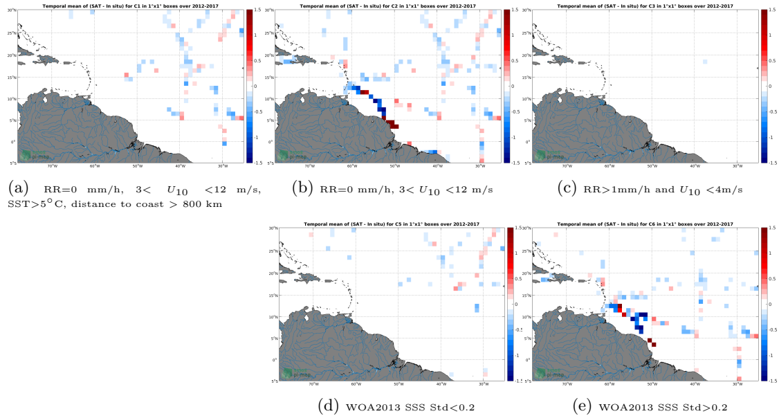
Figure 12: Temporal mean gridded over spatial boxes of size 1^{\circ}\times 1^{\circ} of \Delta SSS (SMOS L3 v317 - Monthly - 25 km (CATDS-CPDC) - TSG-GOSUD-Sailing-ship) for 5 different subdatasets corresponding to:RR=0 mm/h, 3 < U_{10} < 12 m/s, SST >5^{\circ}\text{C} , distance to coast > 800 km (a), RR=0 mm/h, 3 < U_{10} < 12 m/s (b), RR >1 mm/h and U_{10} < 4 m/s (c), WOA2013 SSS Std <0.2 (d), WOA2013 SSS Std >0.2 (e).
