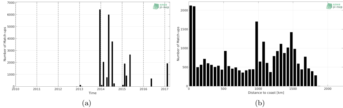
Figure 1: Number of match-ups between TSG-GOSUD-Sailing-ship and SMOS L3 v317 - Monthly - 25 km (CATDS-CPDC) SSS as a function of time (a) and as function of the distance to coast (b) over the Amazon and Orinoco river plumes Pi-MEP region and for the full satellite product period.
