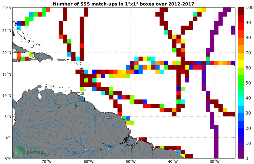
Figure 4: Number of SSS match-ups between TSG-GOSUD-Sailing-ship SSS and the SMOS L3 v317 - Monthly - 25 km (CATDS-CPDC) SSS product for the Amazon and Orinoco river plumes Pi-MEP region over 1°x1° boxes and for the full satellite product period.
