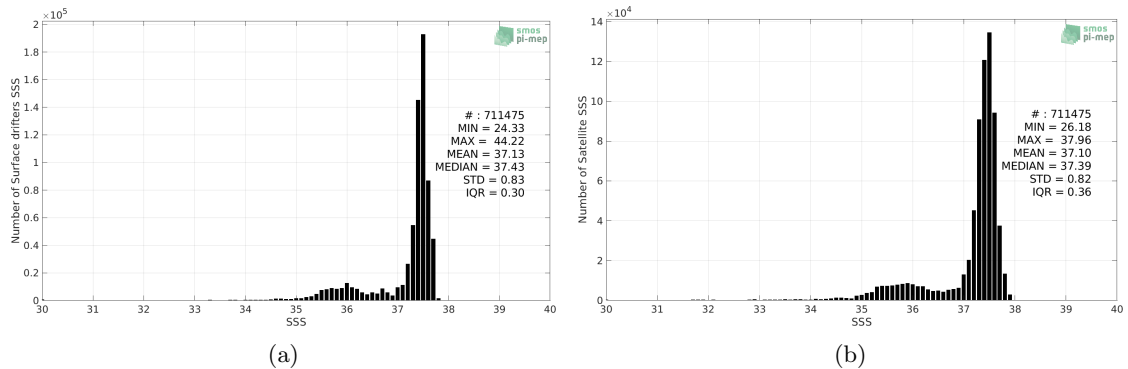
Figure 2: Histograms of SSS from Surface drifters (a) and SMOS SSS L3 v317 - Monthly - 25 km (CATDS-CPDC) (b) considering all match-up pairs per bins of 0.1 over the Amazon and Orinoco river plumes Pi-MEP region and for the full satellite product period.
