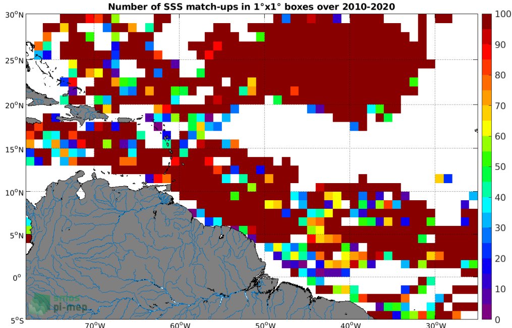
Figure 3: Number of SSS match-ups between Surface drifters SSS and the SMOS SSS L3 v317 - Monthly - 25 km (CATDS-CPDC) SSS product for the Amazon and Orinoco river plumes Pi-MEP region over 1^\circ \times 1^\circ boxes and for the full satellite product period.
