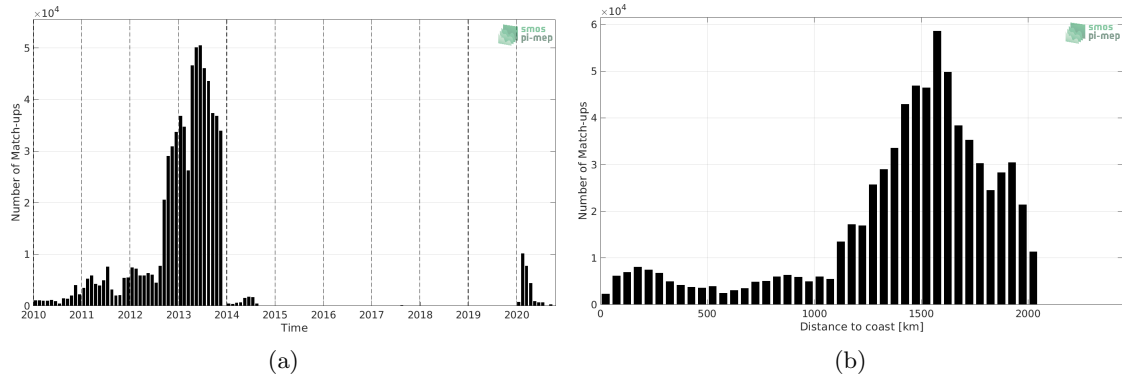
Figure 1: Number of match-ups between Surface drifters and SMOS SSS L3 v317 - Monthly - 25 km (CATDS-CPDC) SSS as a function of time (a) and as function of the distance to coast (b) over the Amazon and Orinoco river plumes Pi-MEP region and for the full satellite product period.
