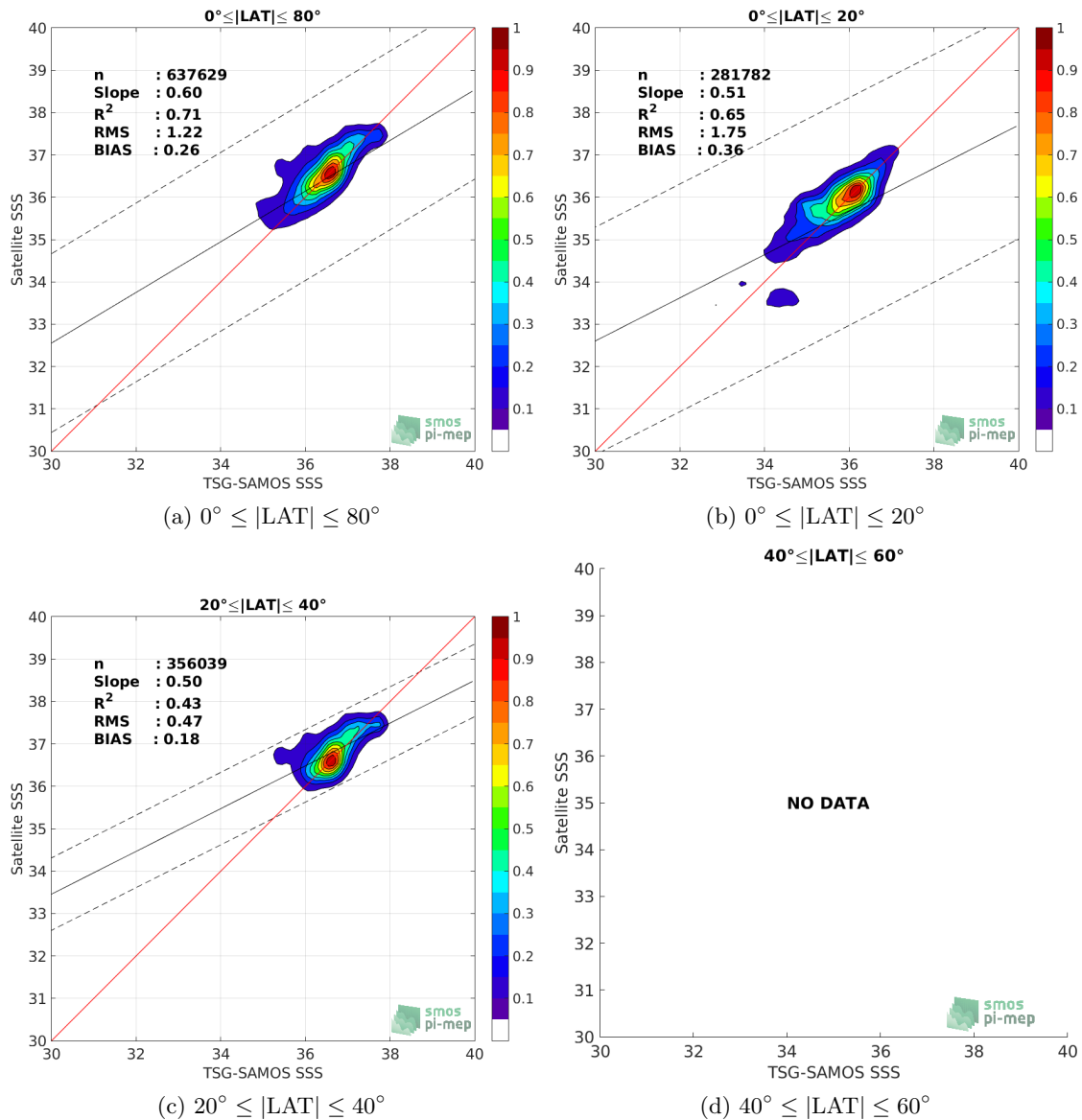
Figure 9: Contour maps of the concentration of SMOS-L3-CATDS-CPDC-V3-MONTHLY-25KM SSS (y-axis) versus TSG-SAMOS SSS (x-axis) at match-up pairs for different latitude bands. For each plot, the red line shows x=y . The black thin and dashed lines indicate a linear fit through the data cloud and the \pm 95\% confidence levels, respectively. The number match-up pairs n , the slope and R^2 coefficient of the linear fit, the root mean square (RMS) and the mean bias between satellite and in situ data are indicated for each latitude band in each plots.
