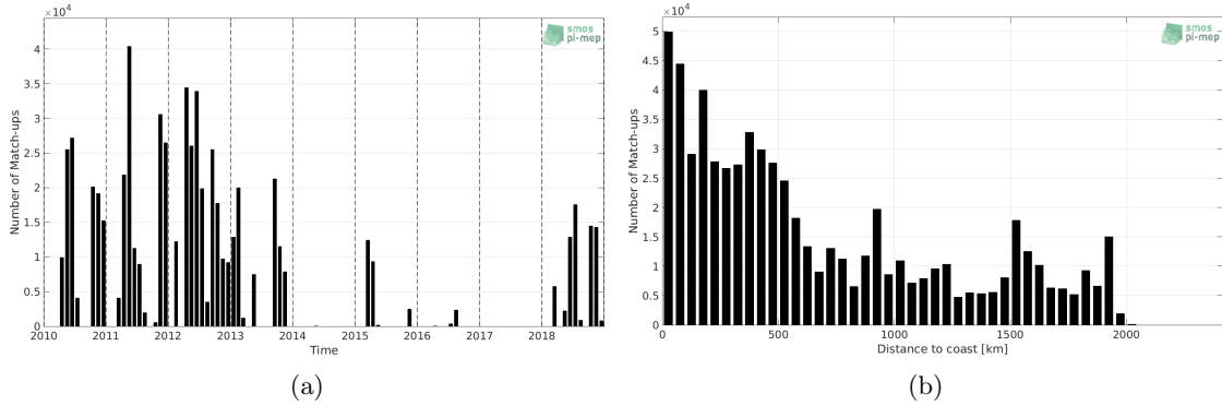
Figure 1: Number of match-ups between TSG-SAMOS and SMOS-L3-CATDS-CPDC-V3-MONTHLY-25KM SSS as a function of time (a) and as function of the distance to coast (b) over the Amazon and Orinoco river plumes Pi-MEP region and for the full satellite product period.
