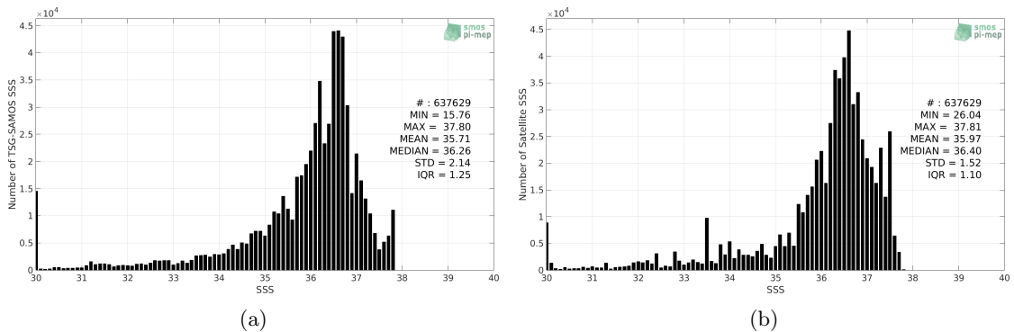
Figure 2: Histograms of SSS from TSG-SAMOS (a) and SMOS-L3-CATDS-CPDC-V3-MONTHLY-25KM (b) considering all match-up pairs per bins of 0.1 over the Amazon and Orinoco river plumes Pi-MEP region and for the full satellite product period.
