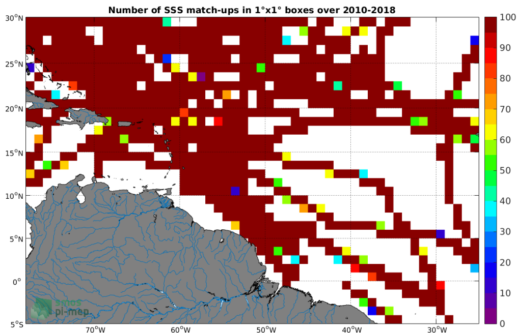
Figure 4: Number of SSS match-ups between TSG-SAMOS SSS and the SMOS-L3-CATDS-CPDC-V3-MONTHLY-25KM SSS product for the Amazon and Orinoco river plumes Pi-MEP region over 1^\circ \times 1^\circ boxes and for the full satellite product period.
