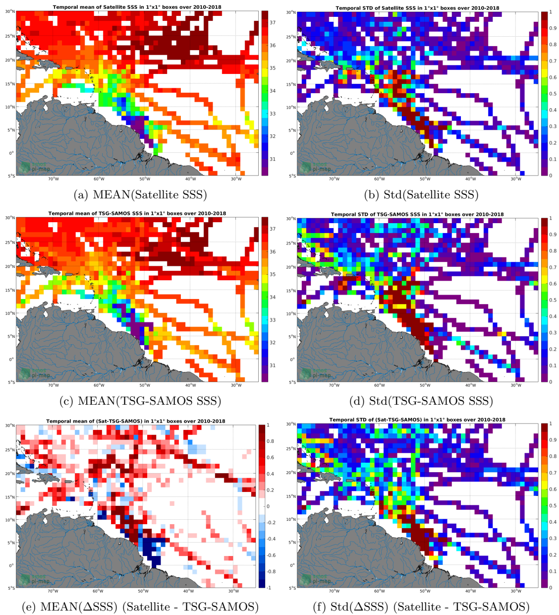
Figure 6: Temporal mean (left) and Std (right) of SSS from SMOS-L3-CATDS-CPDC-V3-MONTHLY-25KM (top), TSG-SAMOS (middle), and of \Delta SSS (Satellite - TSG-SAMOS). Only match-up pairs are used to generate these maps.
