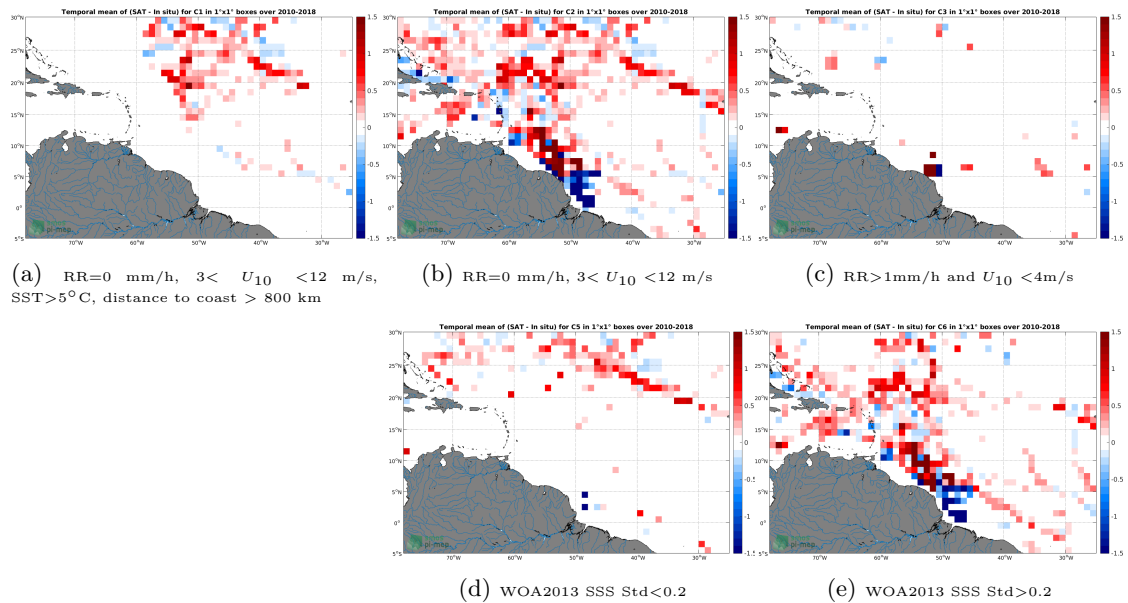
Figure 12: Temporal mean gridded over spatial boxes of size 1^\circ \times 1^\circ of \Delta SSS (SMOS-L3-CATDS-CPDC-V3-MONTHLY-25KM - TSG-SAMOS) for 5 different subdatasets corresponding to: RR=0 mm/h, 3 < U_{10} < 12 m/s, SST >5^\circ\text{C} , distance to coast > 800 km (a), RR=0 mm/h, 3 < U_{10} < 12 m/s (b), RR >1 mm/h and U_{10} < 4 m/s (c), WOA2013 SSS Std <0.2 (d), WOA2013 SSS Std >0.2 (e).
