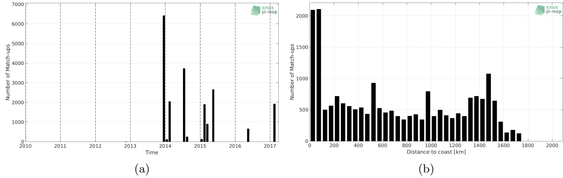
Figure 1: Number of match-ups between TSG-GOSUD-Sailing-ship and SMOS-L3-CATDS-CPDC-V3-MONTHLY-25KM SSS as a function of time (a) and as function of the distance to coast (b) over the Amazon and Orinoco river plumes Pi-MEP region and for the full satellite product period.
