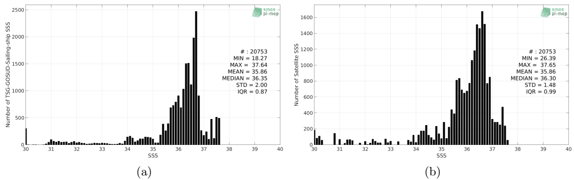
Figure 2: Histograms of SSS from TSG-GOSUD-Sailing-ship (a) and SMOS-L3-CATDS-CPDC-V3-MONTHLY-25KM (b) considering all match-up pairs per bins of 0.1 over the Amazon and Orinoco river plumes Pi-MEP region and for the full satellite product period.
