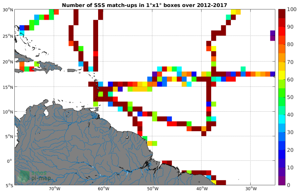
Figure 4: Number of SSS match-ups between TSG-GOSUD-Sailing-ship SSS and the SMOS-L3-CATDS-CPDC-V3-MONTHLY-25KM SSS product for the Amazon and Orinoco river plumes Pi-MEP region over 1°x1° boxes and for the full satellite product period.
