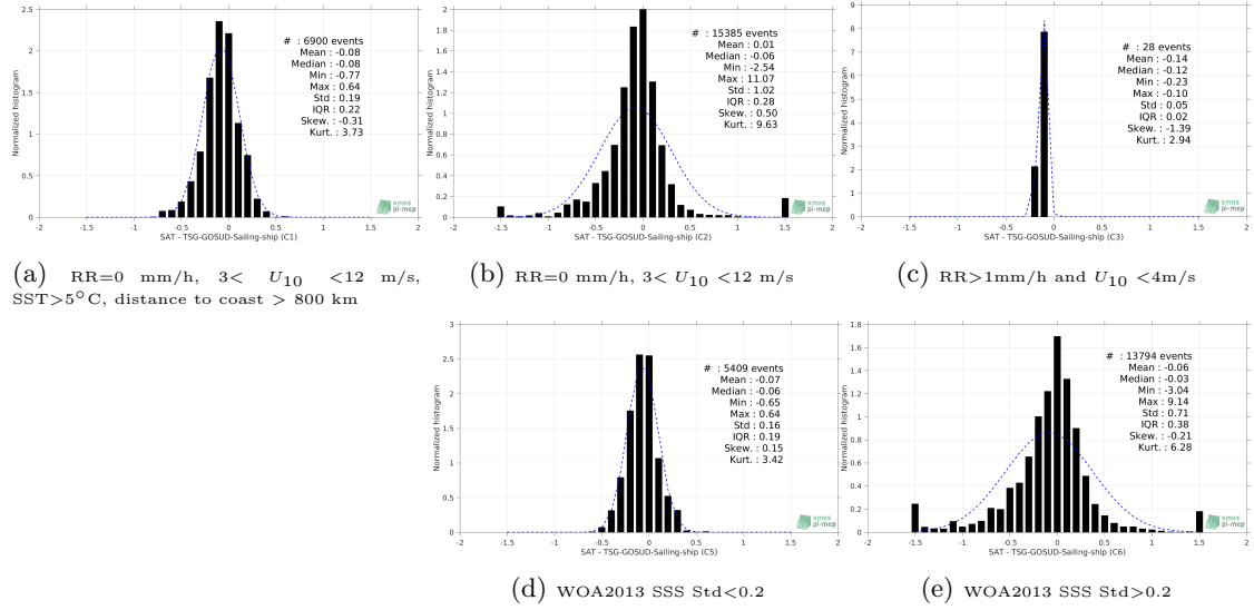
Figure 13: Normalized histogram of \Delta SSS (SMOS-L3-CATDS-CPDC-V3-MONTHLY-25KM - TSG-GOSUD-Sailing-ship) for 5 different subdatasets corresponding to: RR=0 mm/h, 3 < U_{10} < 12 m/s, SST>5°C, distance to coast > 800 km (a), RR=0 mm/h, 3 < U_{10} < 12 m/s (b), RR>1mm/h and U_{10} < 4 m/s (c), WOA2013 SSS Std<0.2 (d), WOA2013 SSS Std>0.2 (e).
