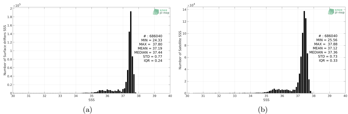
Figure 2: Histograms of SSS from Surface drifters (a) and SMOS-L3-CATDS-CPDC-V3-MONTHLY-25KM (b) considering all match-up pairs per bins of 0.1 over the Amazon and Orinoco river plumes Pi-MEP region and for the full satellite product period.
