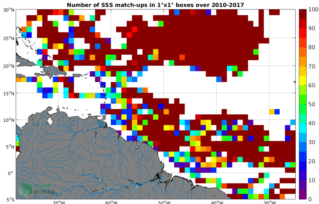
Figure 3: Number of SSS match-ups between Surface drifters SSS and the SMOS-L3-CATDS-CPDC-V3-MONTHLY-25KM SSS product for the Amazon and Orinoco river plumes Pi-MEP region over 1°x1° boxes and for the full satellite product period.
