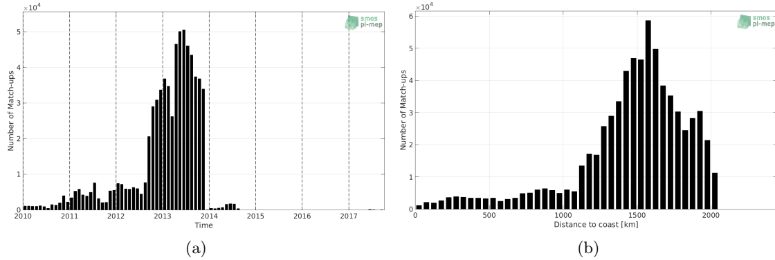
Figure 1: Number of match-ups between Surface drifters and SMOS-L3-CATDS-CPDC-V3-MONTHLY-25KM SSS as a function of time (a) and as function of the distance to coast (b) over the Amazon and Orinoco river plumes Pi-MEP region and for the full satellite product period.
