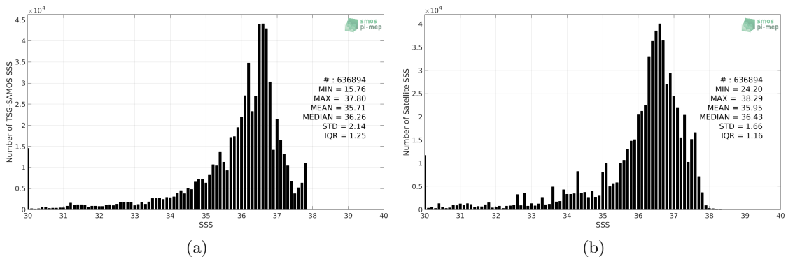
Figure 2: Histograms of SSS from TSG-SAMOS (a) and SMOS-L3-CATDS-CPDC-V3-10DAYS-25KM (b) considering all match-up pairs per bins of 0.1 over the Amazon and Orinoco river plumes Pi-MEP region and for the full satellite product period.
