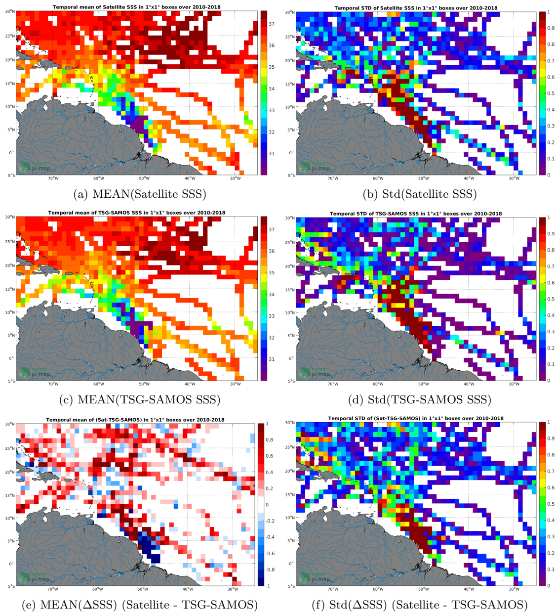
Figure 6: Temporal mean (left) and Std (right) of SSS from SMOS-L3-CATDS-CPDC-V3-10DAYS-25KM (top), TSG-SAMOS (middle), and of \Delta SSS (Satellite - TSG-SAMOS). Only match-up pairs are used to generate these maps.
