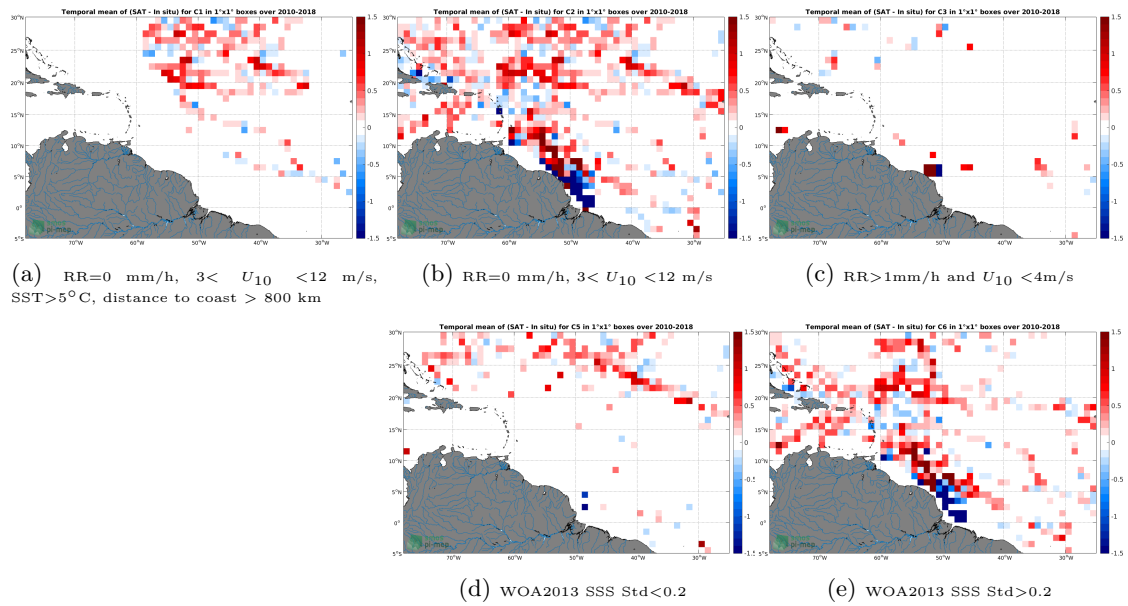
Figure 12: Temporal mean gridded over spatial boxes of size 1^\circ \times 1^\circ of \Delta SSS (SMOS-L3-CATDS-CPDC-V3-10DAYS-25KM - TSG-SAMOS) for 5 different subdatasets corresponding to:RR=0 mm/h, 3 < U_{10} < 12 m/s, SST >5^\circ\text{C} , distance to coast > 800 km (a), RR=0 mm/h, 3 < U_{10} < 12 m/s (b), RR >1 mm/h and U_{10} < 4 m/s (c), WOA2013 SSS Std <0.2 (d), WOA2013 SSS Std >0.2 (e).
