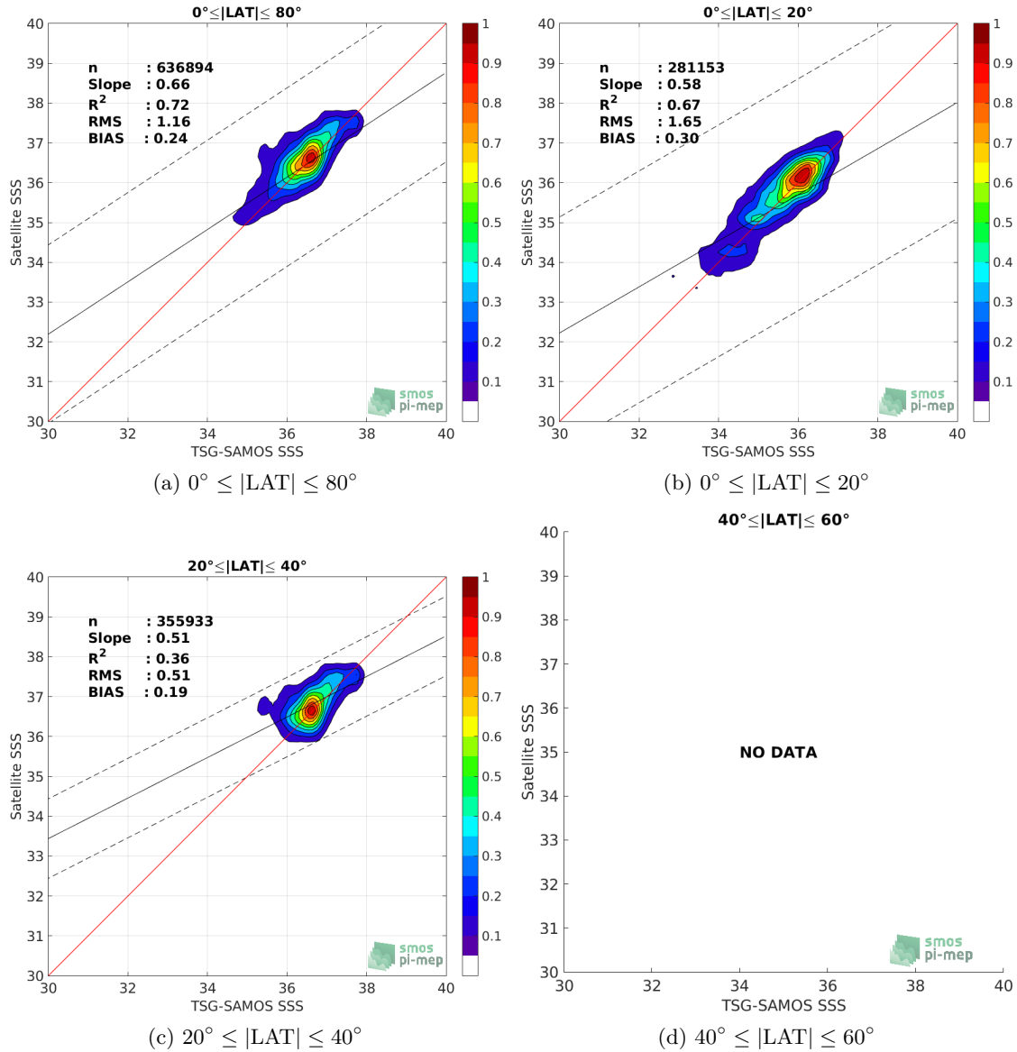
Figure 9: Contour maps of the concentration of SMOS-L3-CATDS-CPDC-V3-10DAYS-25KM SSS (y-axis) versus TSG-SAMOS SSS (x-axis) at match-up pairs for different latitude bands. For each plot, the red line shows x=y . The black thin and dashed lines indicate a linear fit through the data cloud and the \pm 95\% confidence levels, respectively. The number match-up pairs n , the slope and R^2 coefficient of the linear fit, the root mean square (RMS) and the mean bias between satellite and in situ data are indicated for each latitude band in each plots.
