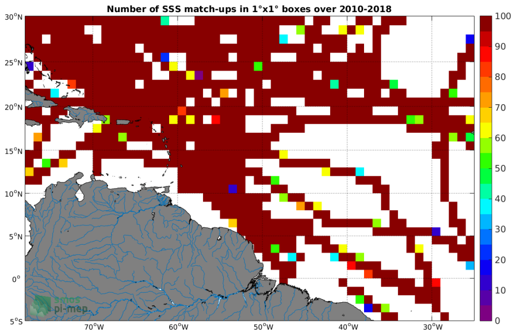
Figure 4: Number of SSS match-ups between TSG-SAMOS SSS and the SMOS-L3-CATDS-CPDC-V3-10DAYS-25KM SSS product for the Amazon and Orinoco river plumes Pi-MEP region over 1^\circ \times 1^\circ boxes and for the full satellite product period.
