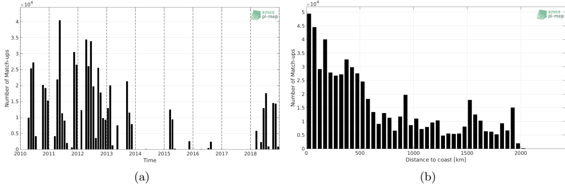
Figure 1: Number of match-ups between TSG-SAMOS and SMOS-L3-CATDS-CPDC-V3-10DAYS-25KM SSS as a function of time (a) and as function of the distance to coast (b) over the Amazon and Orinoco river plumes Pi-MEP region and for the full satellite product period.
