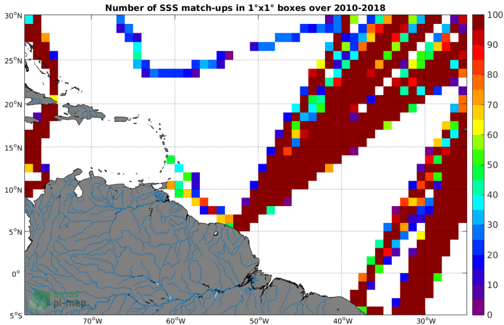
Figure 4: Number of SSS match-ups between TSG-LEGOS-DM SSS and the SMOS-L3-CATDS-CPDC-V3-10DAYS-25KM SSS product for the Amazon and Orinoco river plumes Pi-MEP region over 1°x1° boxes and for the full satellite product period.
