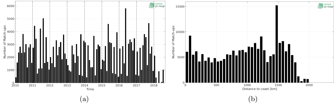
Figure 1: Number of match-ups between TSG-LEGOS-DM and SMOS-L3-CATDS-CPDC-V3-10DAYS-25KM SSS as a function of time (a) and as function of the distance to coast (b) over the Amazon and Orinoco river plumes Pi-MEP region and for the full satellite product period.
