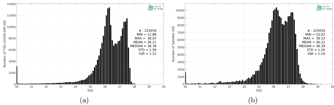
Figure 2: Histograms of SSS from TSG-LEGOS-DM (a) and SMOS-L3-CATDS-CPDC-V3-10DAYS-25KM (b) considering all match-up pairs per bins of 0.1 over the Amazon and Orinoco river plumes Pi-MEP region and for the full satellite product period.
