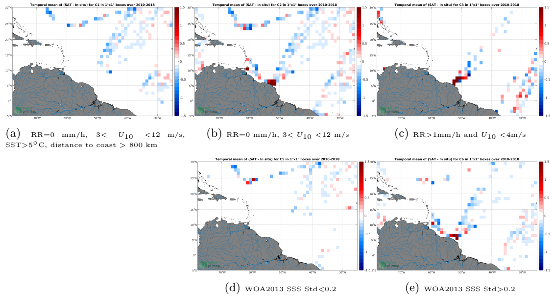
Figure 12: Temporal mean gridded over spatial boxes of size 1^\circ \times 1^\circ of \Delta SSS (SMOS-L3-CATDS-CPDC-V3-10DAYS-25KM - TSG-LEGOS-DM) for 5 different subdatasets corresponding to:RR=0 mm/h, 3 < U_{10} < 12 m/s, SST >5^\circ\text{C} , distance to coast > 800 km (a), RR=0 mm/h, 3 < U_{10} < 12 m/s (b), RR >1 mm/h and U_{10} < 4 m/s (c), WOA2013 SSS Std <0.2 (d), WOA2013 SSS Std >0.2 (e).
